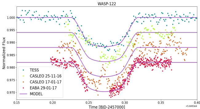
Figure 1: As an example we show for WASP 122 one transit observed by TESS and all our ground-based data, shifted vertically. Our transit model fitting is shown in magenta.
