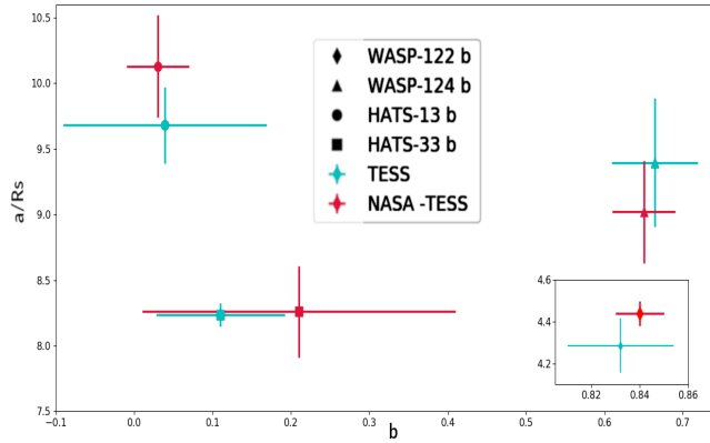
Figure 2: Semi-major axis a/R_s vs impact parameter b . As an example, we show in cyan the results of our analysis on two parameters and the validation results published by NASA in red for all the selected targets.
