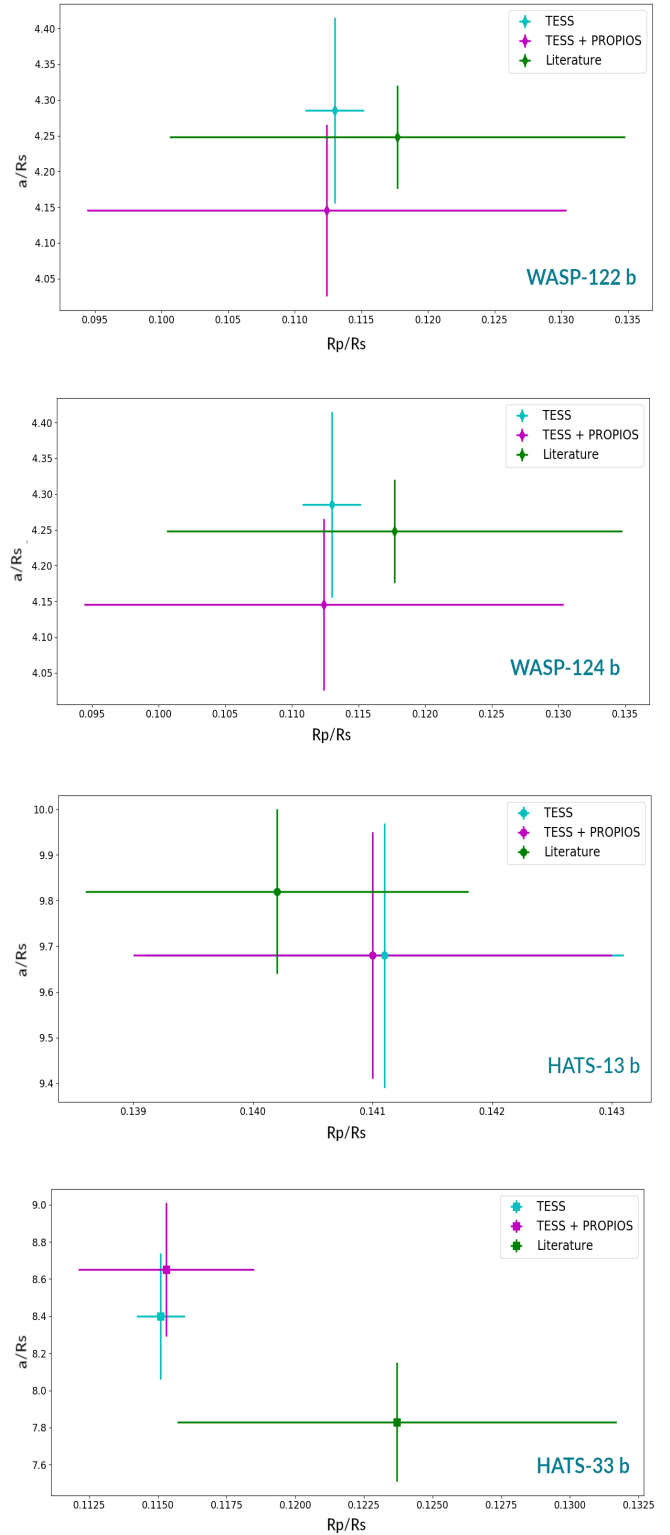
Figure 3: Semi-major axis a/R_s vs planetary radius R_p/R_s . Results for all the exoplanets, taking in account our fit of only TESS data (cyan), TESS + own terrestrial data (magenta), and parameters derived from literature (green).
