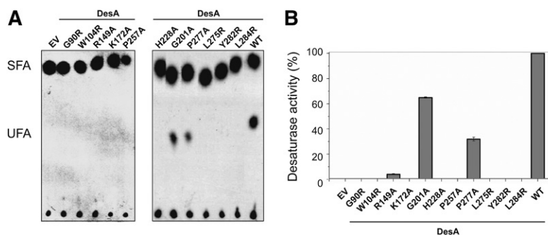
Fig. 4. Essential residues of acyl-lipid desaturases from Firmicutes . A: Autoradiogram of the products of [ ^{14} C] palmitate labeling of B. subtilis strains. Cells were grown overnight at 37°C in MM, washed, resuspended in fresh MM, with or without xylose 0.5%, and labeled with 1 \mu Ci/ml [ ^{14} C]palmitate for 3 h at 37°C. FAs were converted to FAMES and analyzed using 10% silver nitrate-impregnated Silica Gel G plates. The radioactivity on the plates was visualized using a PhosphorImager screen. SFA, saturated fatty acids. B: Desaturase activity of DesA and mutants with single AA substitution expressed in B. subtilis LC5 strain. EV represents the B. subtilis LC5 strain carrying the empty vector. FAMES were prepared from the WT strains and mutants with single AA substitution, and UFAs were quantified by GC/MS. The desaturase activity of DesA was considered as 100%, and UFA production of mutants was expressed as percentage of DesA activity.
