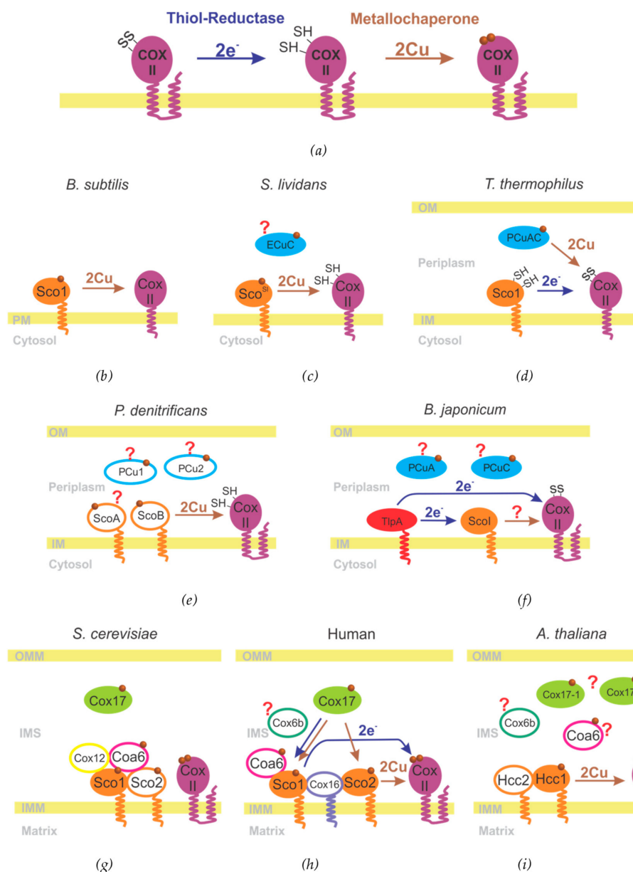
Figure 3. Mechanism of \text{Cu}_A assembly in different organisms. (a) The activities required to assemble the \text{Cu}_A site on newly synthesized COX II. (b–i) Metallochaperone modules in different organisms are indicated from. Proteins from the same families are depicted in the same color. Essential proteins have been colored in filled ovals, and non-essential ones as empty ovals. Arrows indicate the function of each proteins, when assigned.
