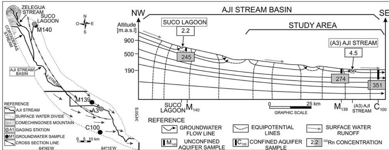
Figure 8 | Cross section of a groundwater-surface water relationship scheme taking into account 222 Rn values.
