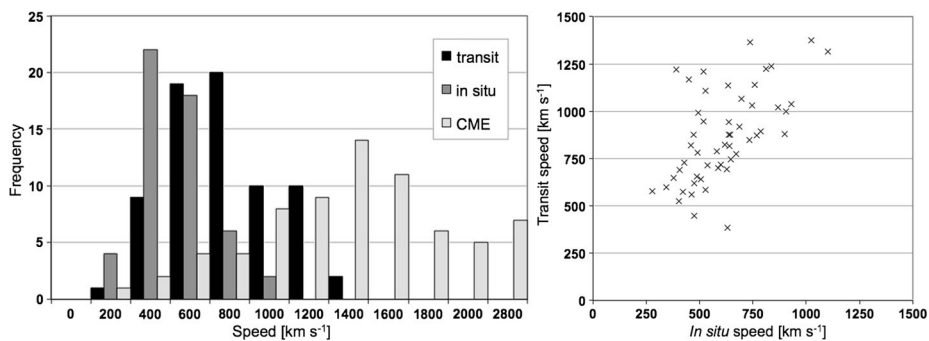
Figure 7 Left: Speed distribution in bins of 200 km s -1 , with the shock-transit speed in black columns, the in-situ shock speed in dark gray, and CME projected speed in light-gray columns. Right: shock-transit speeds (vertical axis) vs. in-situ shock speeds (horizontal axis) for 52 out of the 71 events.
