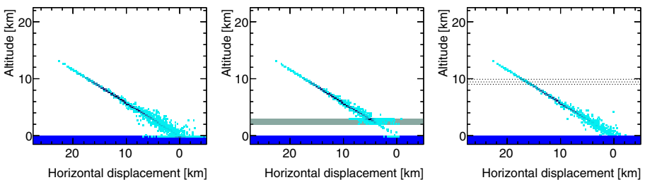
Fig. 1 Schematic view of EAS geometry for \Theta = 60^\circ in the different atmospheric conditions. The left panel shows the observed photon distribution projected on SDP for the clear atmosphere condition. The middle and right panels are same but for the cloudy cases of large optical depth at 3 km and of small optical depth at 10 km, respectively
