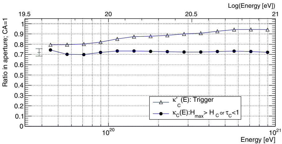
Fig. 5 Ratio of the geometrical aperture for averaged cloudy condition to that from clear atmosphere as a function of energy [11]. The triangles and circles show \kappa'_C and \kappa_C defined in Eqs. (4) and (5), respectively. In the latter case, H_C < H_{\max} or \tau_C < 1 are required for triggering EAS events. The error bar denotes an estimated uncertainty on \kappa_C
