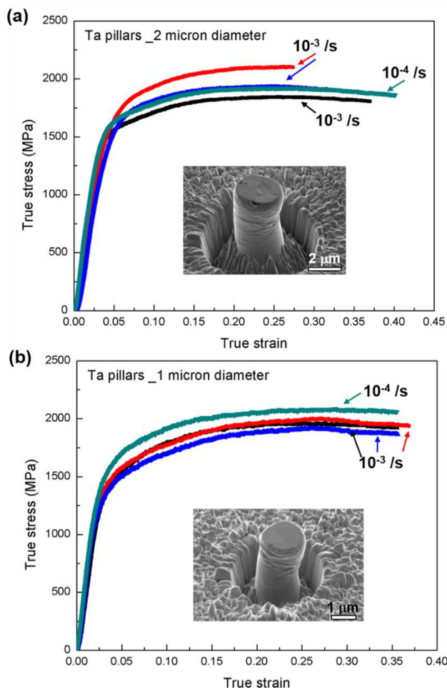
Fig. 2 – Stress strain curves for two different pillar diameters (1 and 2 \mu\text{m} ) and two strain rates ( 10^{-3} and 10^{-4} \text{s}^{-1} ). The results of two tests under each condition are shown. The effects of pillar diameter and of strain rate are small.
