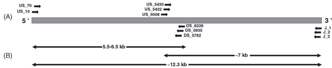
Fig. 2. Schematic representation of L-RT-PCR strategies. Primer locations and lengths of L-RT-PCR products are given. A: Position of the primers relative to genomic RNA. B: Relative position of LD-PCR amplicons. Primer sequences are given in Table 2.
