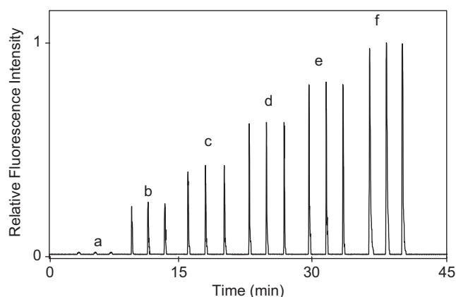
Fig. 3. Calibration curve of sildenafil. Standard solution of sildenafil: (a) 0.00 \mu\text{g mL}^{-1} ; (b) 1.00 \mu\text{g mL}^{-1} ; (c) 2.00 \mu\text{g mL}^{-1} ; (d) 3.00 \mu\text{g mL}^{-1} ; (e) 4.00 \mu\text{g mL}^{-1} ; and (f) 5.00 \mu\text{g mL}^{-1} . \lambda_{\text{exc}}=310 nm; \lambda_{\text{em}}=430 nm. Excitation and emission slit widths are 3 nm and 5 nm, respectively.
