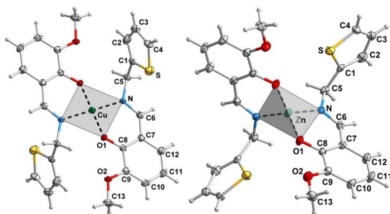
Figure 1: View of [\text{Cu}(\text{oVATPNH}_2)_2] ( \text{CuL}_2 ) (left) and [\text{Zn}(\text{oVATPNH}_2)_2] ( \text{ZnL}_2 ) (right) showing the labeling of the non-H atoms and their displacement ellipsoids at the 30% probability level. The unlabeled atoms are obtained from the labeled ones through a crystallographic inversion center at the copper location and by a 180° rotation around a two-fold axis passing through the zinc ion, respectively. Metal-ligand bonds are indicated by dashed lines. For clarity, in both complexes only it is shown the dominant conformer of the rotationally disordered thiophene group.
