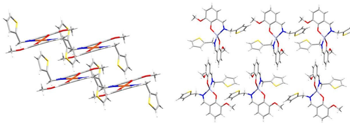
5 6 7 8 9 10 11 12 13 14 15 16 17 18 19 20 21 22 23 24 25 26 27 28 29 30 31 32 33 34 35 36 37 38 39 40 41 42 43 44 45 46 47 48 49 50 51 52 53 54 55 56 57 58 59 60 Figure 2. Crystal packing of \text{CuL}_2 (left) and \text{ZnL} (right)
