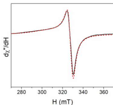
Figure 4. EPR spectrum of [\text{Cu(oVATPNH2)}_2] ( \text{CuL}_2 ) at 150 K (solid line) together with the best fit (dashed line). Experimental details: modulation amplitude 0.1 mT, time constant 40.96 ms, conversion time 327.68 ms, gain 1 \times 10^3 (short ranges) or 1 \times 10^4 (long 0 – 700 mT ranges) and power 20 mW. Microwave frequency 9.4260 GHz.
