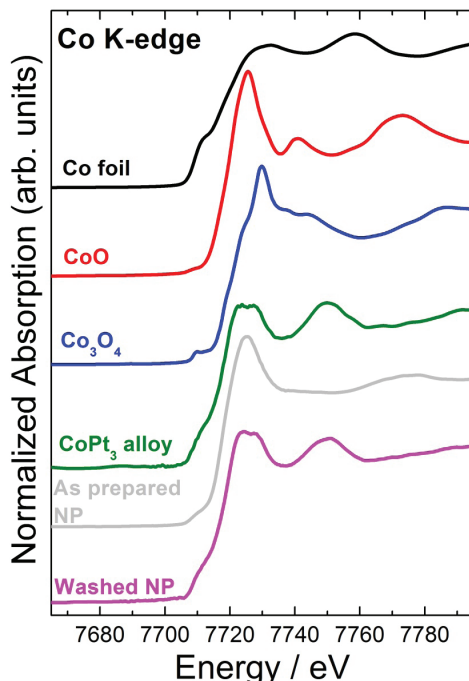
Figure 2. XANES spectra at the Co-K edge of as-prepared and washed samples compared to metallic Co foil, CoO, Co 3 O 4 and CoPt 3 alloy reference compounds. Note the energy edge position of samples coincident with metallic Co foil reference and the similarity between the washed sample and the CoPt 3 alloy reference compound.
