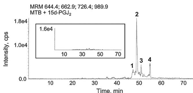
Fig. 8. MRM experiments with control and 15d-PG 2 -treated microtubules samples. MRM experiments from tryptic, 15d-PG 2 -modified peptides 1–4. The inset shows the MRM results for the corresponding control microtubules sample.
