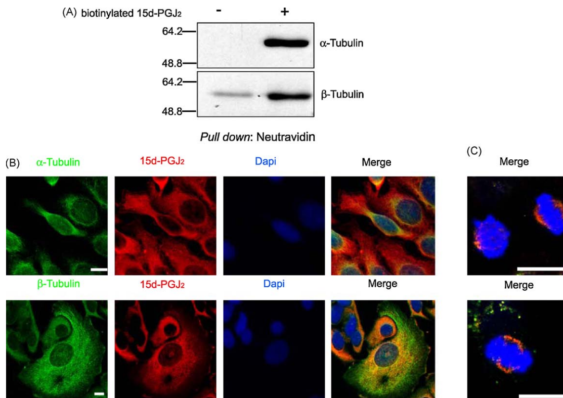
Fig. 6. Binding of biotinylated 15d-PGJ 2 to \alpha - and \beta -tubulin in vivo . (A) MCF-7 cells were incubated or not with biotinylated 15d-PGJ 2 for 2 h and cell lysates were subjected to pull-down assays with Neutravidin-gel beads. The presence of \alpha - and \beta -tubulin was assessed by Western blot analysis with specific antibodies. (B) MCF-7 cells were treated as in A and cellular accumulation of biotinylated 15d-PGJ 2 was evaluated by confocal microscopy. Tubulin was detected with a specific mouse monoclonal antibody and 15d-PGJ 2 with an anti-biotin antibody. Scale bar, 10 \mu m. (C) Same staining as in B, showing colocalization of biotinylated 15d-PG 2 in mitotic cells. Scale bar, 20 \mu m.
