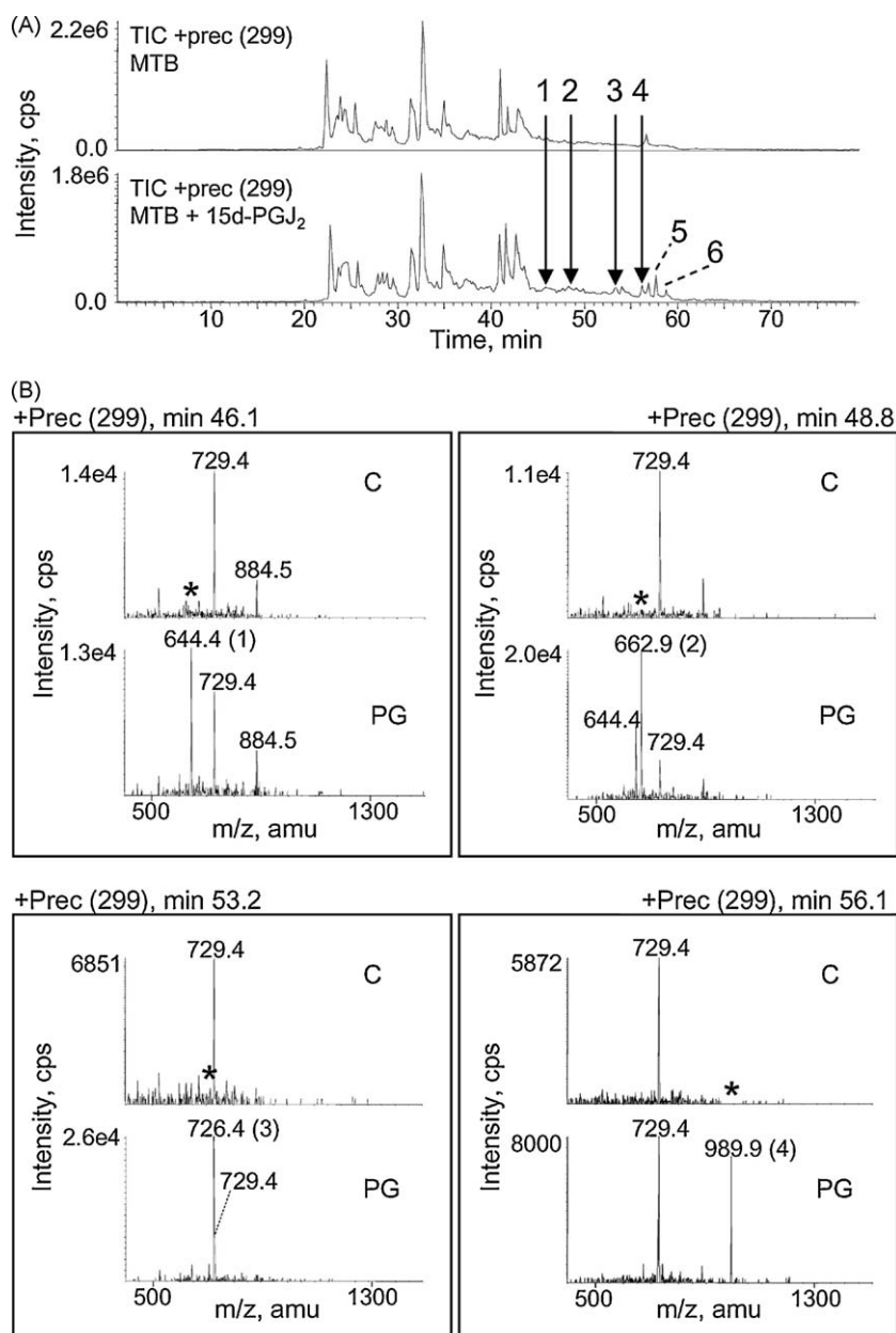
Fig. 7. MS analyses of 15d-PG 2 binding to microtubules. Total ion chromatogram (TIC) of the precursor ion scanning of fragment at m/z 299.4 from control (A, upper panel) or 15d-PG 2 -treated (A, lower panel) microtubules samples, digested with trypsin. Arrows labeled as 1–4 indicate retention times corresponding to different peptide mass composition between control and 15d-PG 2 -treated microtubules samples. These differences are detailed in (B) with labels 1–4 indicating the 15d-PG 2 -modified sequences. C means control-, and PG means 15d-PG 2 -treated microtubule samples. Differential masses absent in the control mass spectrum are labeled as an (*). Peaks 5 and 6 correspond to differential chromatographic peaks. Peak 5 contains the peptide with sequence 309-HGKYMACC PG LLYR-320 (one missed cleavage at K311). Peak 6 corresponds to the 15d-PG 2 dimer.
