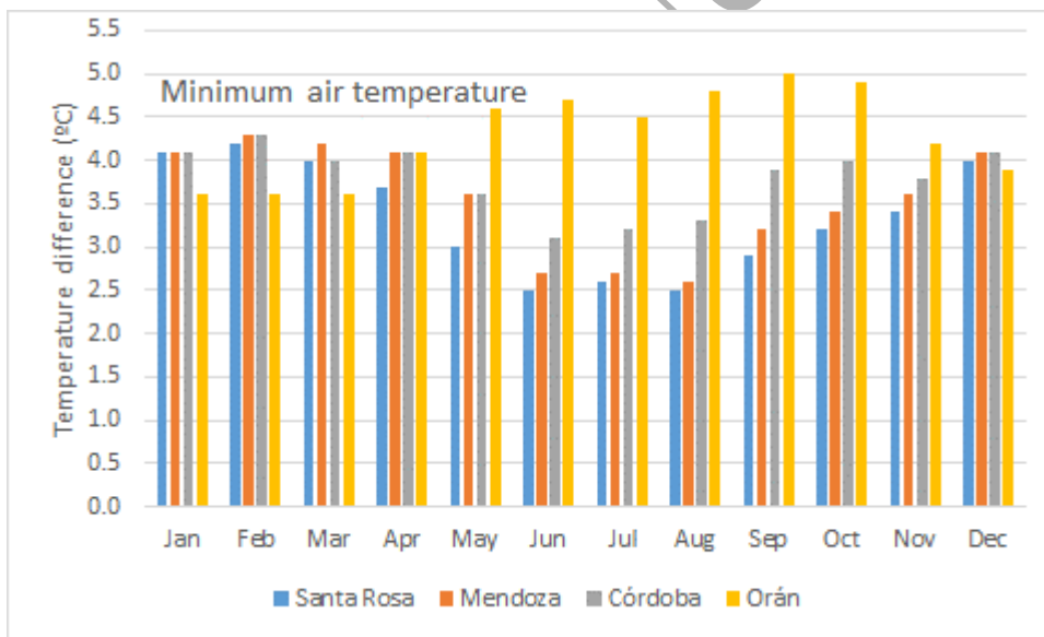
Figure 6: Temperature difference of the minimum air temperature, between monthly average in 2080 and monthly average in the period 1961-1990, for the four sites.
