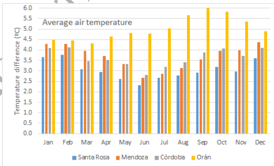
Figure 4: Temperature difference of the average air temperature, between monthly average in 2080 and monthly average in the period 1961-1990, for the four sites.
