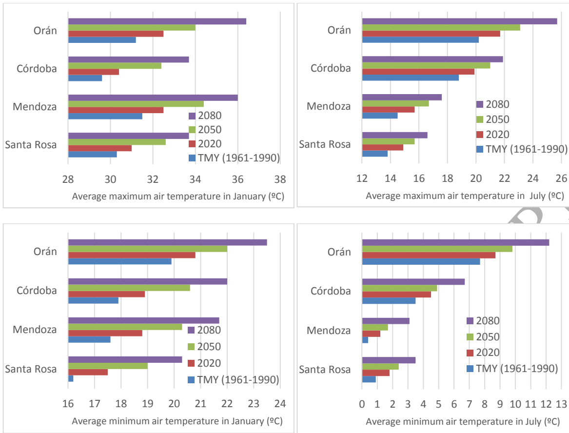
Figure 7: Mean, maximum and minimum air temperatures for January (left) and July (right), for years 2020, 2050 and 2080. TMY is also shown as a reference.
