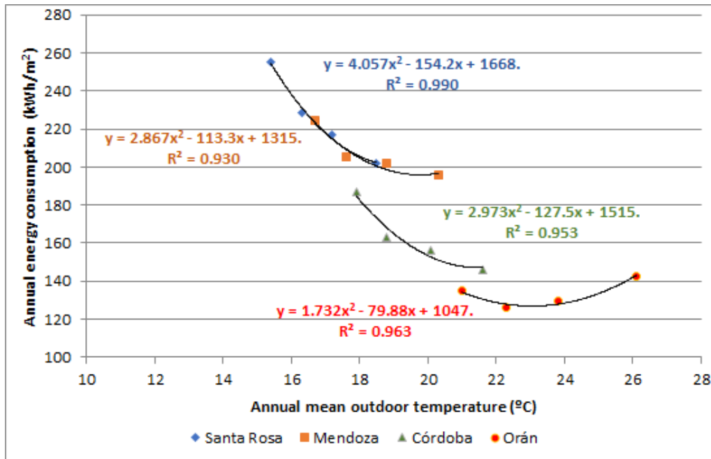
Figure 10: annual energy consumption per square meter versus annual mean temperature, for the four periods (TMY, 2020, 2050 and 2080) and for each site.
