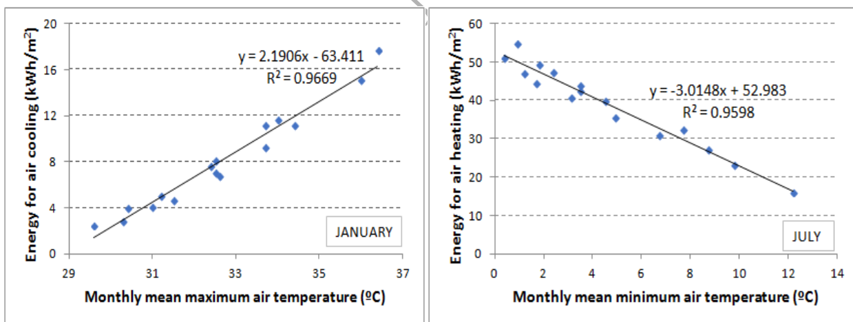
Figure 9: energy consumption for air cooling versus monthly mean maximum outdoor air temperature in summer (January, left) and energy consumption for air heating versus monthly mean minimum outdoor air temperature in winter (July, right), per square meter, for the case-study building in the four cities and for the four periods (TMY, 2020, 2050 and 2080).
