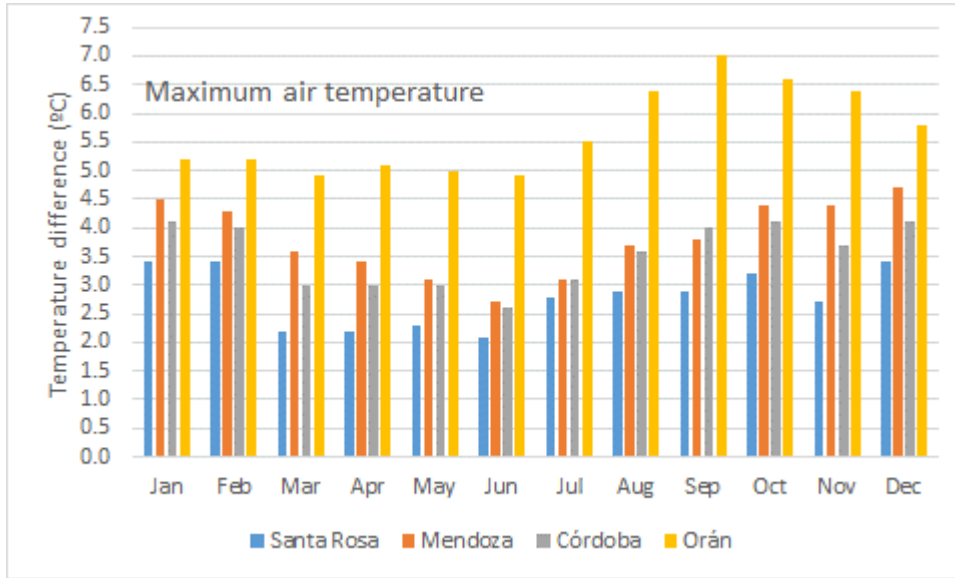
Figure 5: Temperature difference of the maximum air temperature, between monthly average in 2080 and monthly average in the period 1961-1990, for the four sites.
