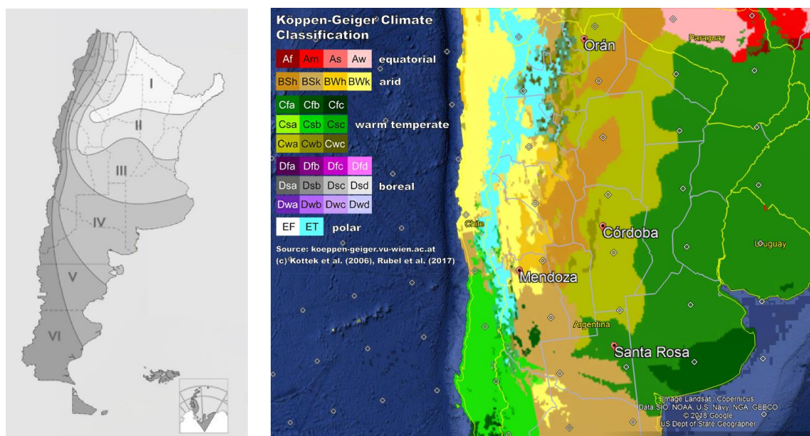
Figure 2: Argentinean bioclimatic regions (IRAM Norm 11603 [21]) (left) and view in Google Earth of the Köppen climate classification [22] (right) together with HADCM3 grid points and the final set of cities used in this study.
