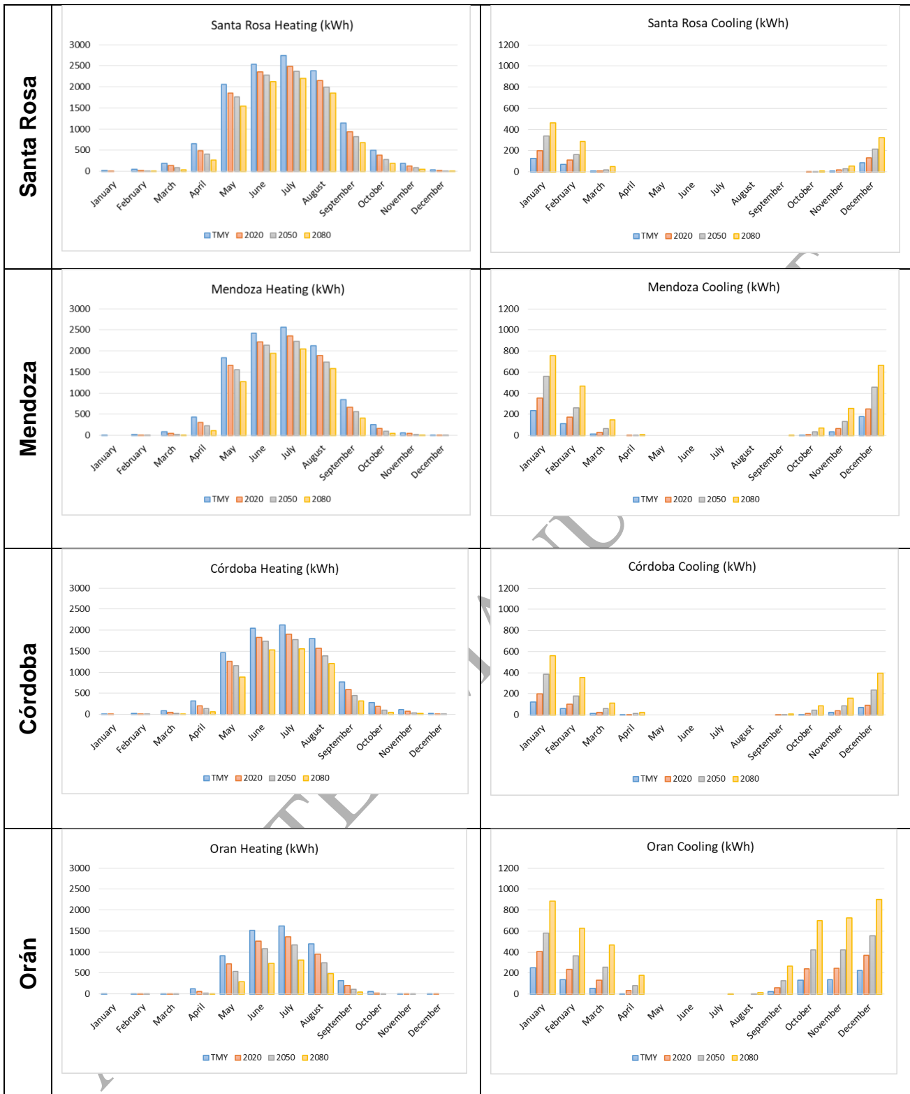
Figure 8: monthly energy consumption for TMY, 2020, 2050 and 2080 in the four sites, for the case-study.
