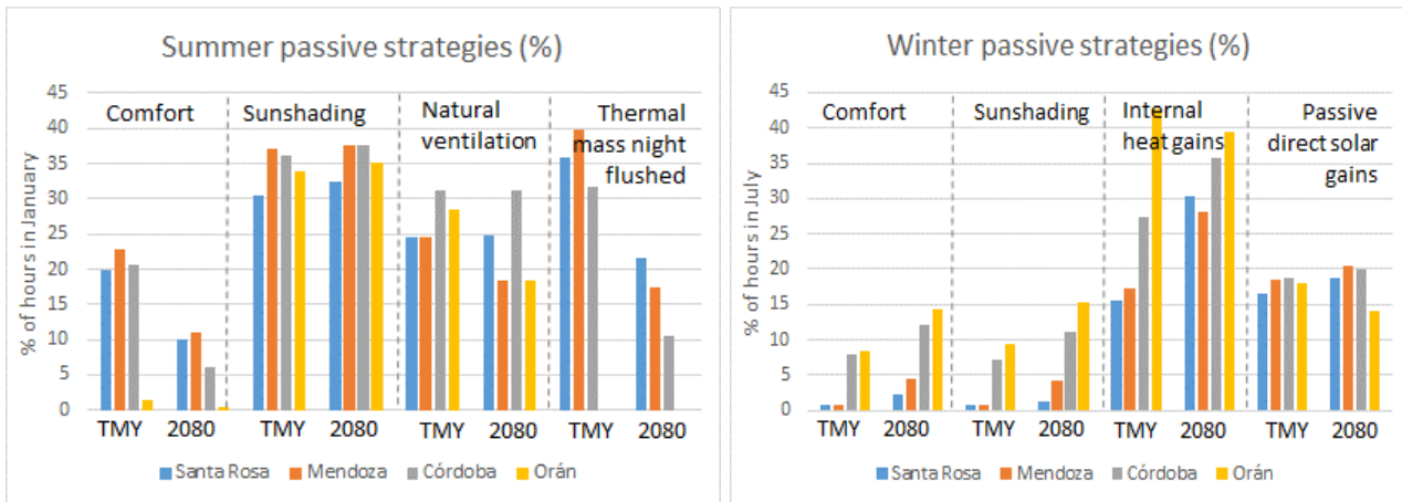
Figure 11: Percentage of hours in a month when design passive strategies can be used, for the four sites, in TMY (1961-1990) and in 2080.
