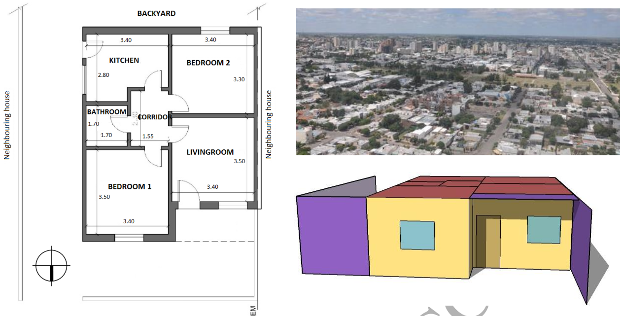
Figure 3. Plan view (left), SketchUp model of the house designed for EnergyPlus and urban environment in Santa Rosa (right).
