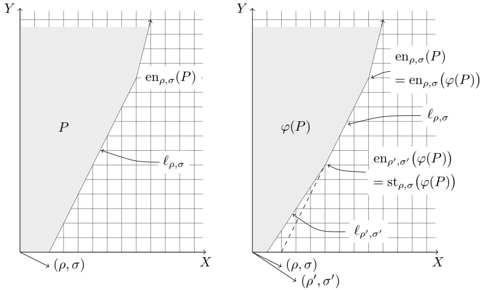
FIGURE 6. Illustration of Proposition 5.3
