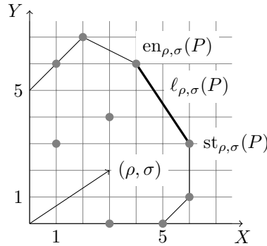
FIGURE 1. Illustration of st and en
