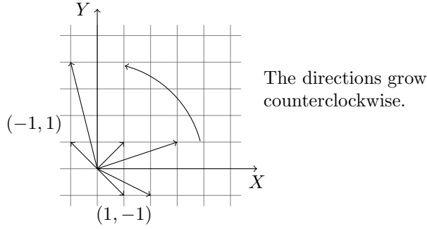
FIGURE 3. Order relation in \overline{\mathfrak{D}} .
