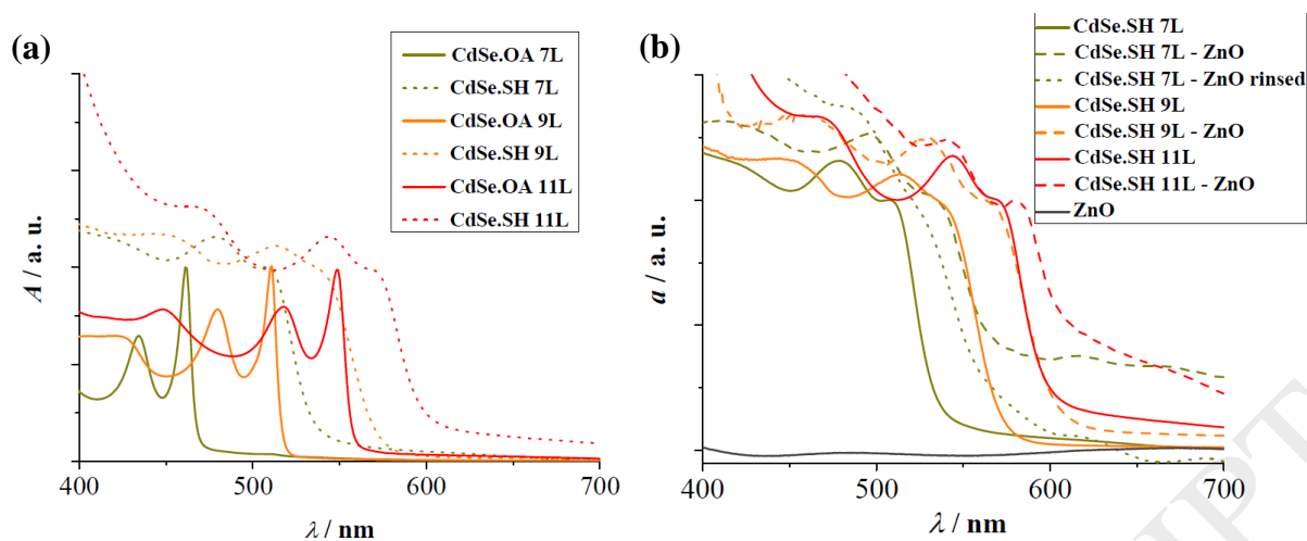
Figure 1. UV-VIS absorption spectra of (a) CdSe NPLs of different thicknesses (7, 9 and 11 layers). The NPLs passivated by OA are indicated in full lines, while NPLs after ligand exchange with \text{SH}^- are shown as dotted lines. (b) Spectra of the 7, 9 and 11 layers thick CdSe.SH NPLs in dispersion (indicated by green, orange and red full lines, respectively) and after attachment to ZnO nanorod arrays (indicated by dashed lines of the corresponding color, and by a dotted line after consequent washing with ethanol). Bare ZnO nanorod arrays are represented by a grey full line.
