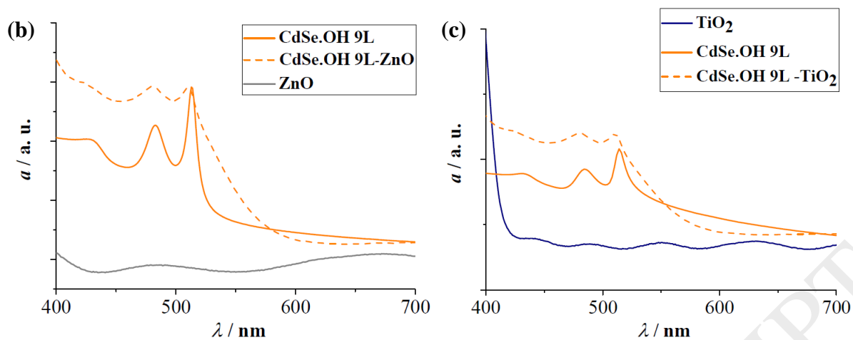
Figure 4. UV-VIS absorption spectra of (a) 9 layers thick CdSe NPLs before and after ligand exchange with OH - (indicated by full and dotted lines, respectively). (b) ZnO NR arrays and 9 layers thick CdSe.OH NPLs in dispersion (indicated by orange full lines), as well as after attachment to ZnO NR arrays (indicated by orange dashed lines). (c) TiO 2 NR arrays and 9 layers thick CdSe.OH NPLs in dispersion (indicated by orange full lines) and after attachment to TiO 2 NR arrays (indicated by orange dashed lines)
