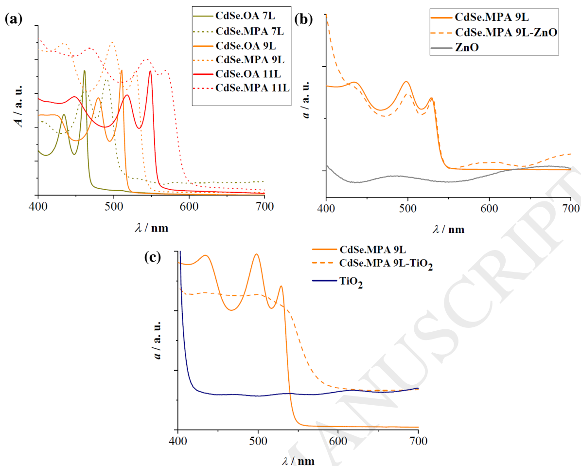
Figure 6. UV-VIS absorption spectra of (a) 7, 9 and 11 layers thick CdSe NPLs before and after ligand exchange with MPA (indicated by green, orange and red full and dotted lines, respectively). (b) ZnO NR arrays and 9 layers thick CdSe.MPA NPLs in dispersion (indicated by orange full lines) and after attachment to ZnO NR arrays (indicated by orange dashed lines). (c) TiO 2 NR arrays and 9 layers thick CdSe.MPA NPLs in dispersion (indicated by orange full lines) and after attachment to TiO 2 NR arrays (indicated by orange dashed lines)
