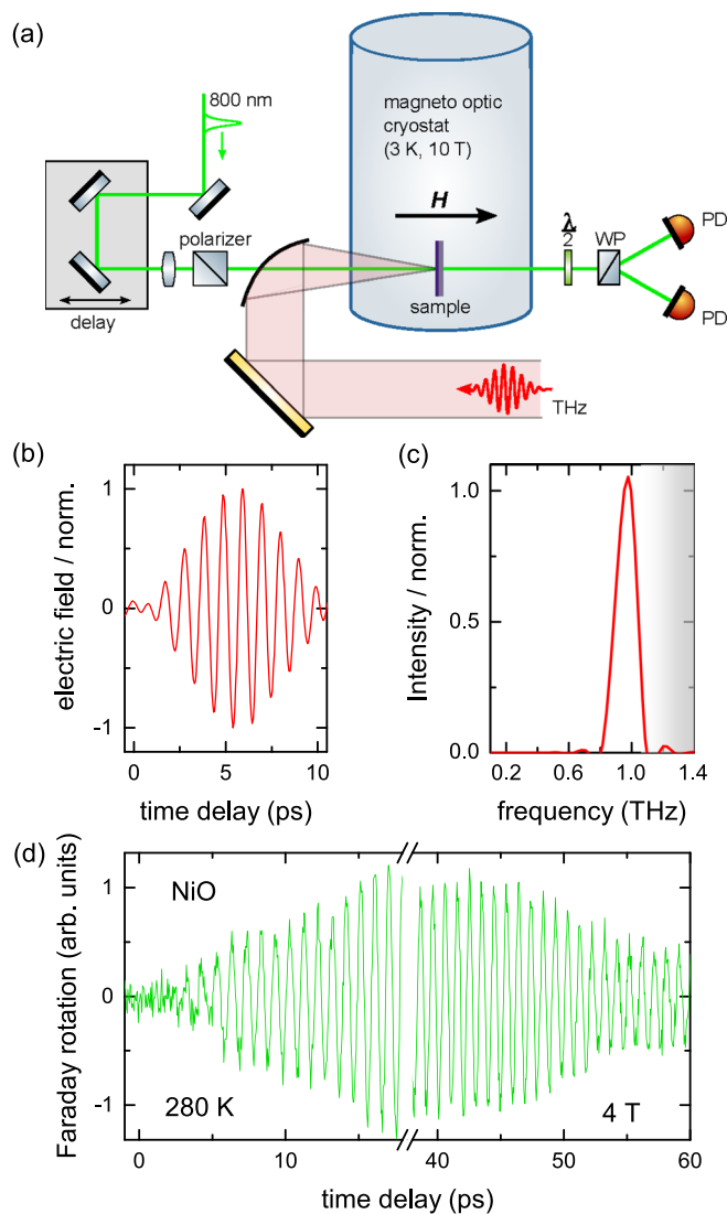
FIG. 2. (a) Experimental endstation for THz pump Faraday probe experiments at the TELBE facility. 16,17 Tunable narrow-band/multicycle THz pulses (red) are focused on the sample at normal incidence. Transient changes of the magnetization are probed by Faraday rotation of pulses from a collinear Ti:Sapphire based femtosecond laser (green) that can be timed to the THz pulses to better than 12 fs resolution. 18 \frac{1}{2} WP, and PD denote half-wave plate, Wollaston prism, and photodiode detector, respectively. (b) Electric field of the utilized 1 THz pump pulses and (c) the corresponding spectrum obtained from Fourier transformation. (d) Typical transient Faraday measurement in an applied magnetic field of 4 T obtained at 280 K. The coherent oscillation of the magnetization is probed by the determination of the polarization change.
