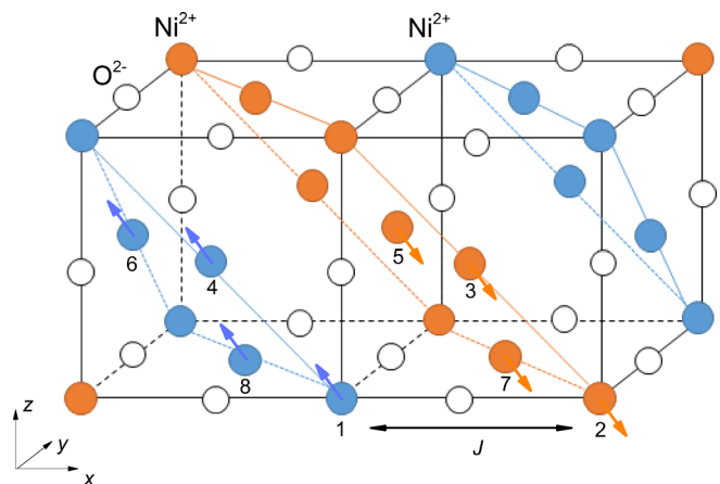
FIG. 1. Illustration of the crystallographic and magnetic structure of NiO. Antiferromagnetic structure consists of ferromagnetically aligned spins in the \{111\} planes which are alternately stacked along the perpendicular direction. Below T_N , spins of the \text{Ni}^{2+} ions are along the \langle 112 \rangle directions, as indicated by the arrows. Eight simple cubic sublattices of Ni spins are indicated by the numbers marked at the origin of each sublattice. The dominant spin interaction is the superexchange between the next-nearest-neighbor \text{Ni}^{2+} ions via the 180^\circ \text{Ni}^{2+}-\text{O}^{2-}-\text{Ni}^{2+} configuration as denoted by J .
