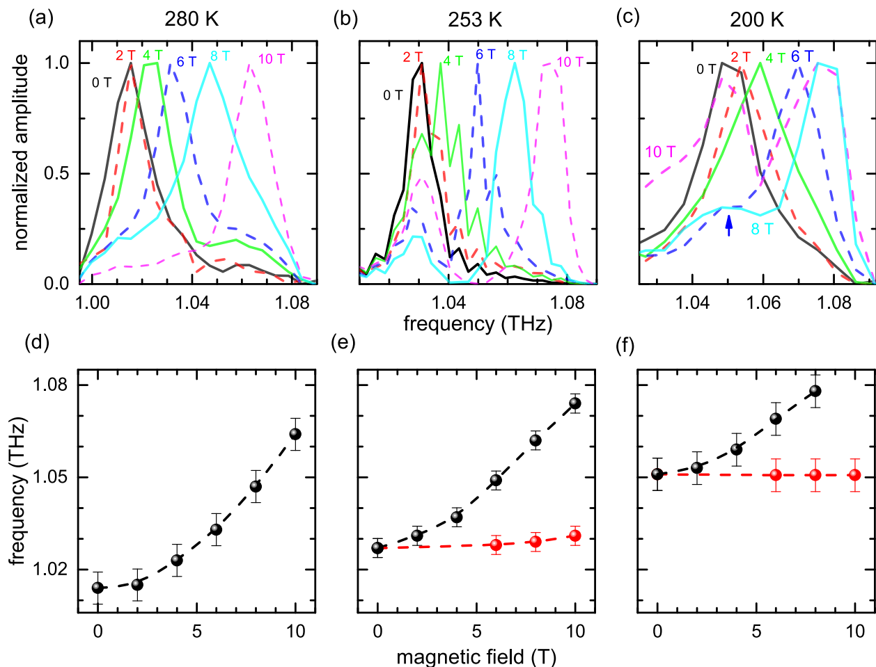
FIG. 4. Magnetic field dependence at (a) and (d) 280 K, (b) and (e) 253 K, and (c) and (f) 200 K. While only one mode is observed at 280 K, at the lower temperatures two modes are resolved. The qualitatively different field-dependencies of the two modes are in agreement with the predicted behaviors for mode A and mode B [see Fig. 5 and Eq. (1)]. In (d)–(f), the dashed lines are guides to the eyes.
