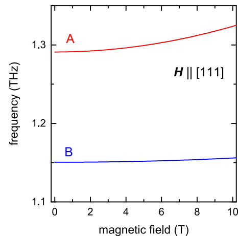
FIG. 5. Field dependence of the higher-energy spin modes mode A at 1.29 THz (red) and mode B at 1.15 THz (blue) obtained from the eight-sublattice model [Eq. (1)], for the external magnetic field applied along the [111] direction.
