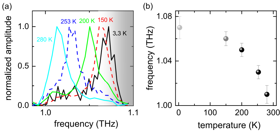
FIG. 3. (a) Amplitude spectra obtained from Fourier transformation of the time-domain signals of Faraday rotation angle at various temperatures. The shaded area in the high-frequency limit indicates the spectral range where the THz radiation is strongly reduced by water absorption. (b) Temperature dependence of the peak frequencies in (a). Error bars indicate the apparent full widths at the half maxima.
