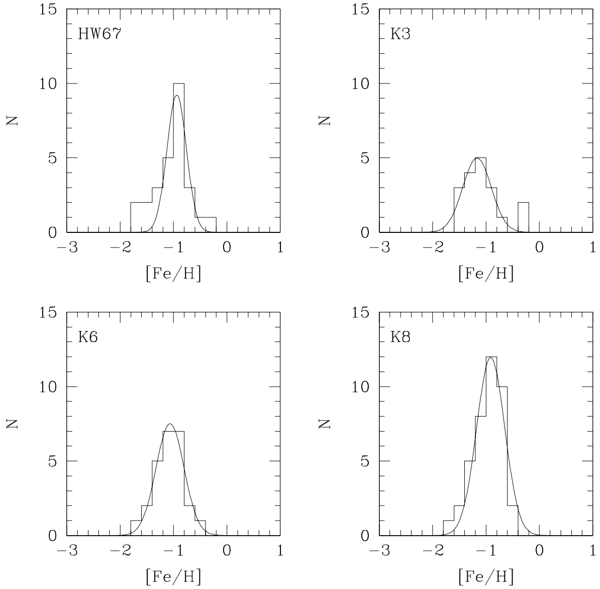
Fig. 5.— Same as Figure 4 but for stars surrounding clusters HW67, K3, K6 and K8.
