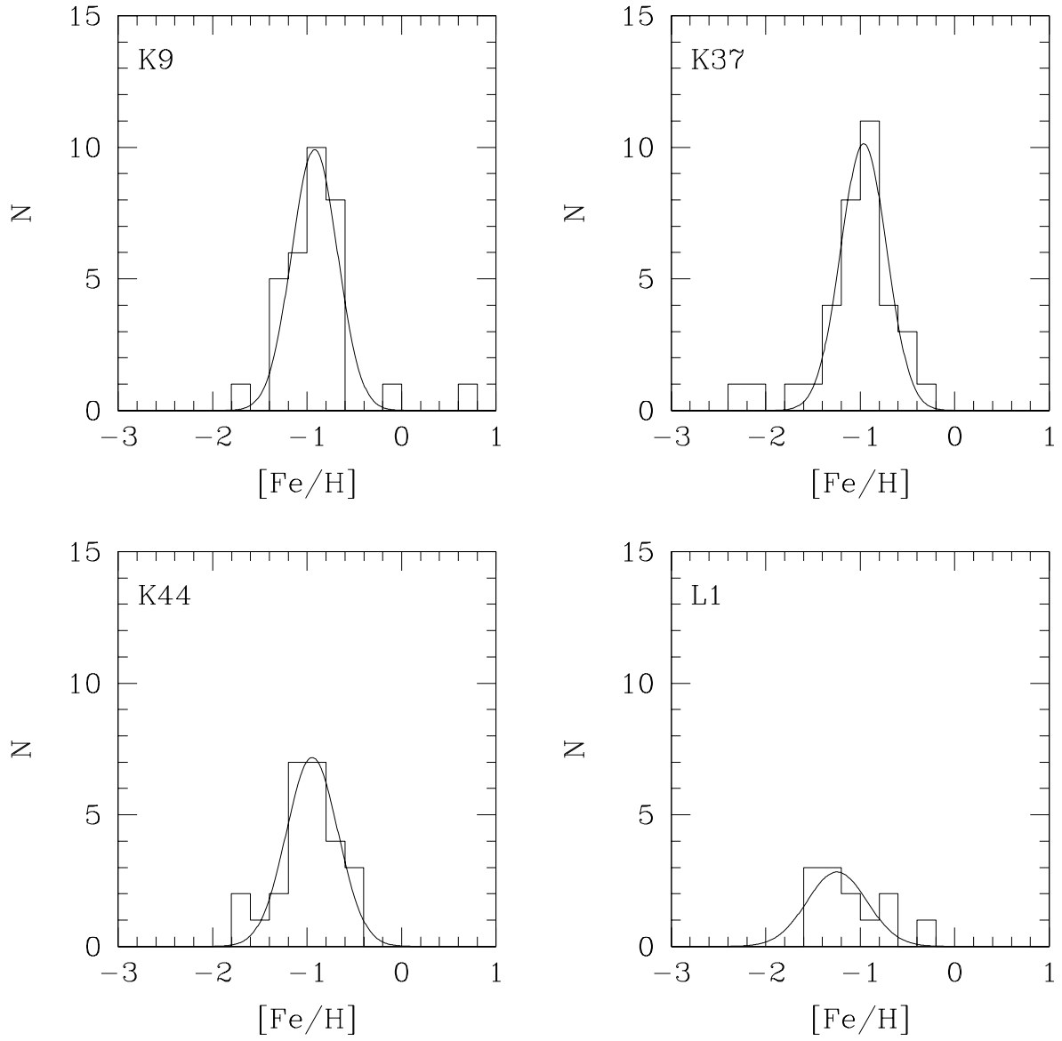
Fig. 6.— Same as Figure 4 but for stars surrounding clusters K9, K37, K44 and L1.
