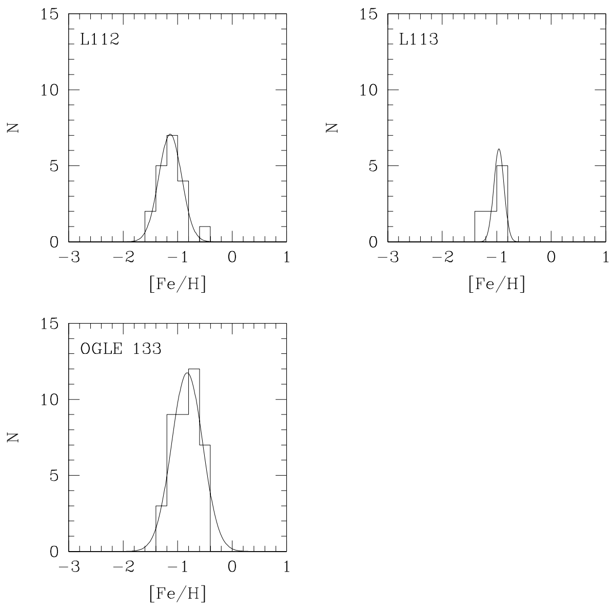
Fig. 7.— Same as Figure 4 but for stars surrounding clusters L112, L113 and OGLE 133.
