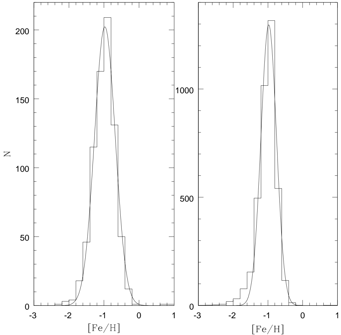
Fig. 2.— Metallicity distribution of all 750 SMC field red giants studied in the present work and P10 (Left panel) and of our field giants plus 3037 giants studied by D14b (Right panel). In both figures the solid curve is the best Gaussian fit, which is generally a very good representation of the MD except for the most metal-poor stars, where there is a hint of an excess of stars in the observed MD.
