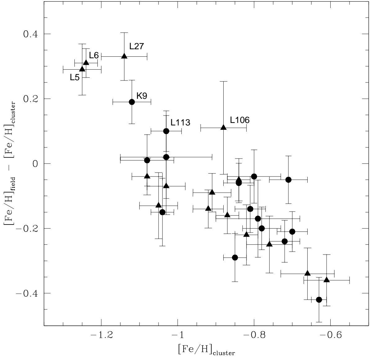
Fig. 10.— Difference between field and cluster metallicities as a function of cluster metallicity. Symbols are the same as Figure 8
