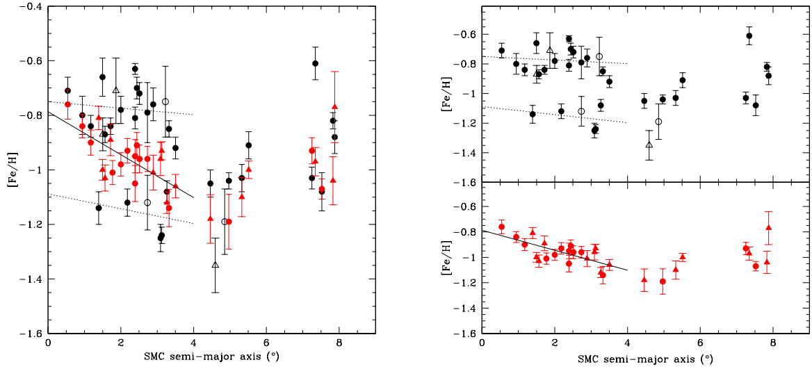
Fig. 11.— Left panel. Metallicities as a function of the semi-major axis a . Black and red symbols represent cluster and surrounding field metallicities, respectively. Cluster sample: filled circles represent clusters studied in P09 and P15, open circles and triangles those from Da Costa & Hatzidimitriou (1998) and Glatt et al. (2008a,b), respectively. The field sample symbols are the same as in Figure 8. Field median metallicities are plotted. The solid line corresponds to the best linear fit performed considering only field stars, while dotted lines are the linear fit considering separately the two groups of clusters (metal-rich and metal-poor groups). Right panel. Same as the left panel. The two stellar populations (clusters above and fields below) are separated for a better visualization of the two dataset.
