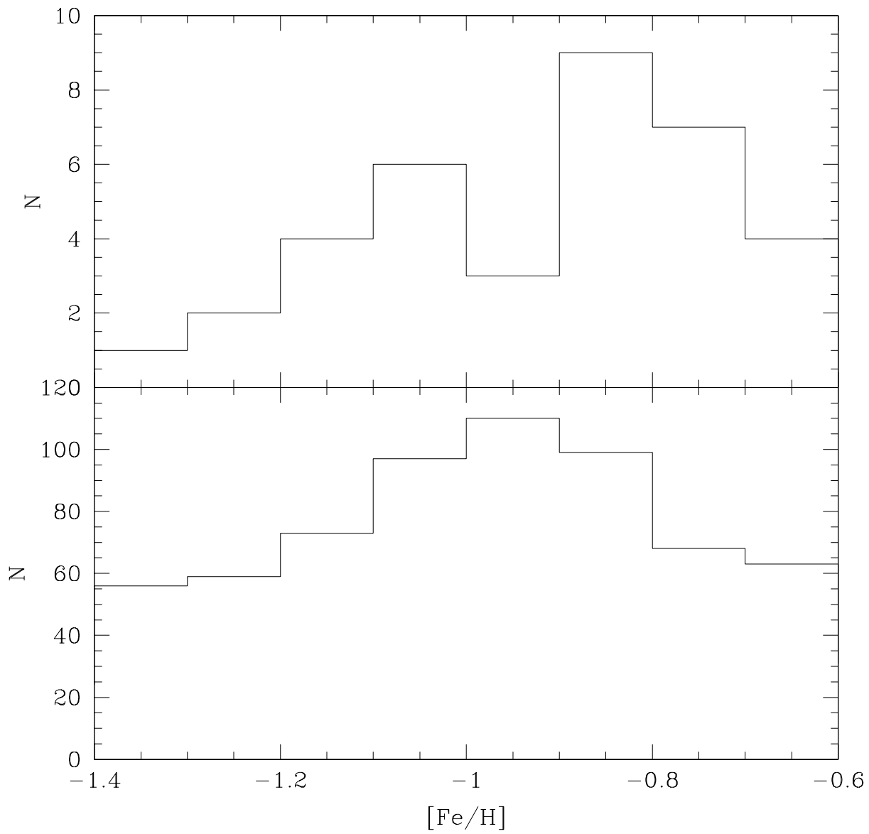
Fig. 3.— Metallicity distribution of our field giants (bottom) compared to the cluster metallicity distribution from P15 (top).
