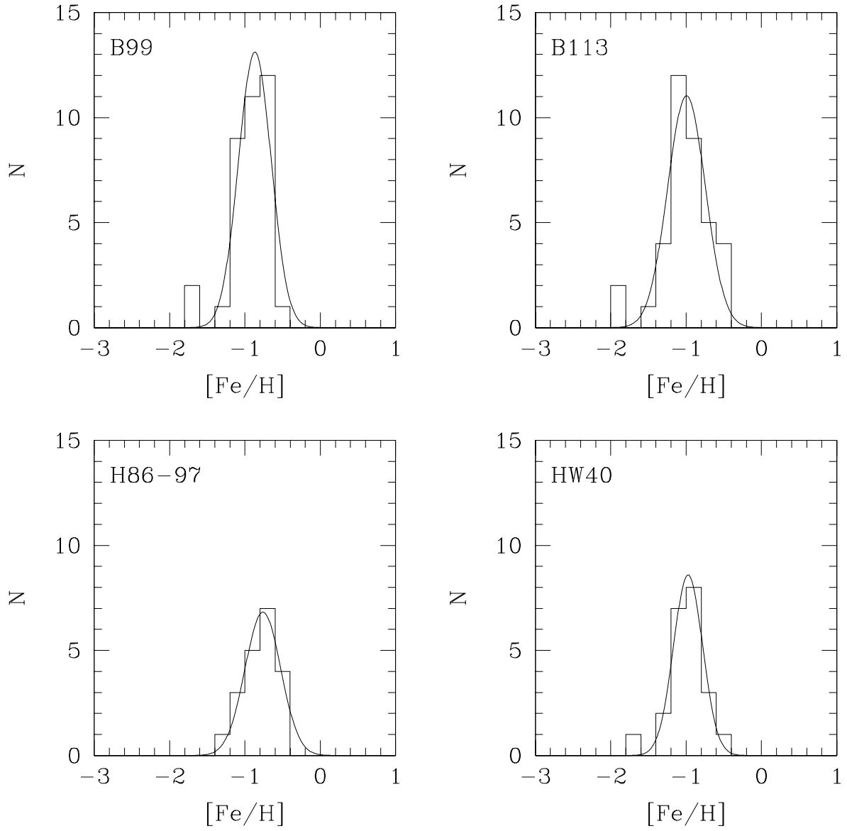
Fig. 4.— Metallicity distributions of the field stars surrounding clusters B99, B113, H86-97 and HW40. The corresponding Gaussian fits are shown in solid lines.
