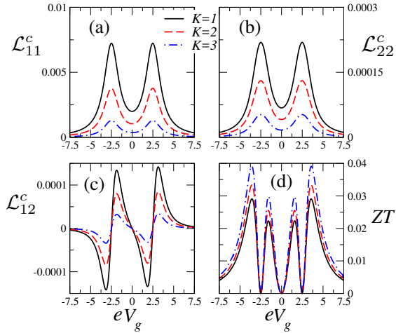
FIG. 5: Onsager coefficients (panels (a), (b) and (c)) and figure of merit ZT (panel (d)) corresponding at the charge heat engine or refrigerator at the temperature k_B T = 0.1\gamma and magnetic field B = 5\gamma/\mu_B and \theta = 0 , as functions of the gate voltage. Other details are the same as in the previous Fig.
