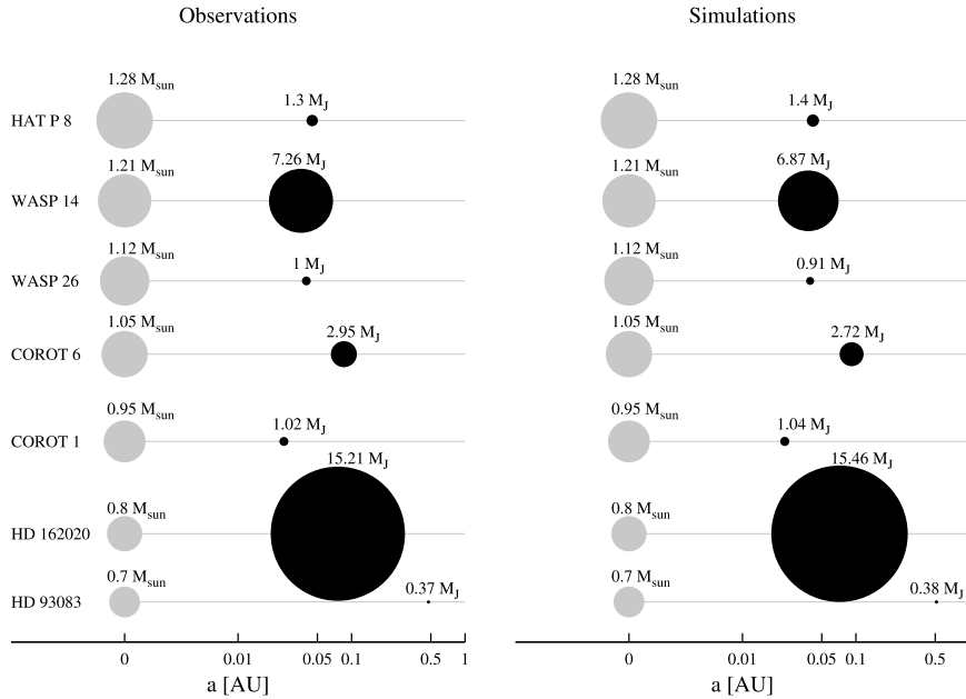
Figure 1. The figure shows some examples of hot and warm Jupiter systems with a single planet observed, shown in the first column, compared with similar hot and warm Jupiter systems generated in our simulations (second column). The semi-major axis is shown in the abscissa, while the size of the circle indicates the planet’s mass, which is also printed in Jupiter masses ( M_J ) above each planet.
