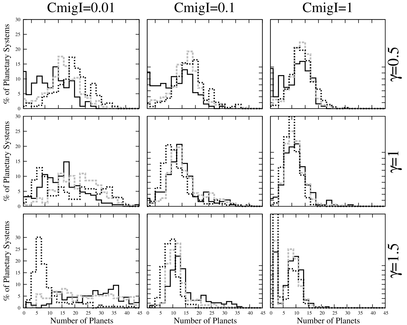
Figure 8. The figure shows histograms which represent the number of planets harboured per low-mass planetary system. In each histogram, the simulation results are separated into three categories: planetary systems formed in low-mass discs (solid line), planetary systems formed in intermediate-mass discs (grey dotted line) and planetary systems formed in massive discs (black dotted line). The rows show the results found when different initial disc profiles are assumed ( \gamma = 0.5, 1 and 1.5 ) and the columns show the numerical results when we assume different migration rates, c_{\text{migl}} = 0.01, 0.1 and 1 .
