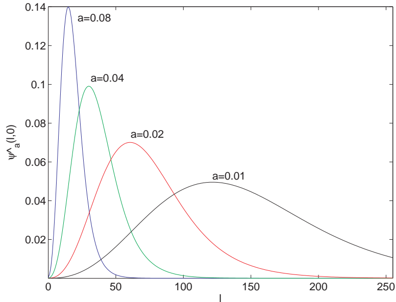
Figure 2: Behavior of \hat{\psi}_a(l, 0) as a function of the scale a . If a = 0.01 , the bandwidth of the dilated wavelet exceeds the limit fixed by the discretization.
