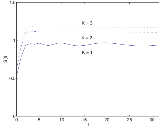
Figure 4: The function S(l) for l \in [0, 31) and K = 1, 2, 3 . First Approach.
