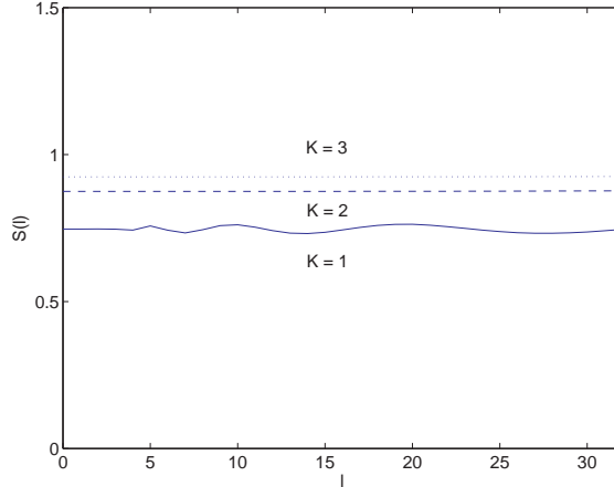
Figure 5: The function S(l) for l \in [0, 31[ and K = 1, 2, 3 . Second Approach. ■
