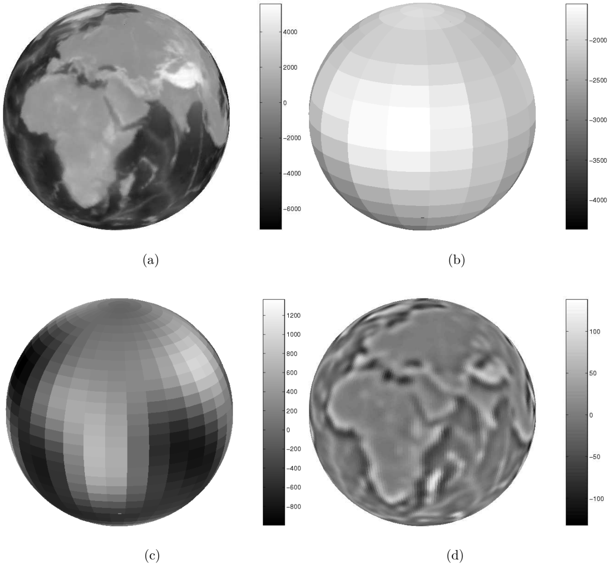
Figure 6: Decomposition of the Earth elevation map. (a) Global average elevation data ( 512 \times 512 equi-angular grid). The elevations are relative to the mean level of the oceans (in meter). (b) W_0[p, q] . (c) W_3[p, q] . (d) W_6[p, q] .
