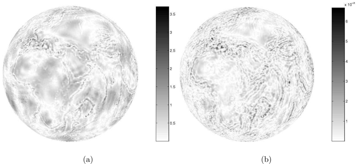
Figure 7: (a) Difference between the elevation map f and its approximation Lf . (b) Difference between f and its reconstruction f^{(3)} obtained after three iterations of the conjugate gradient algorithm. For (a) and (b), the values are in percentage of the maximum value of the original data.
