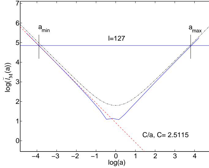
Figure 3: \check{l}_M(a) as a function of a in solid line (logarithmic representation).
