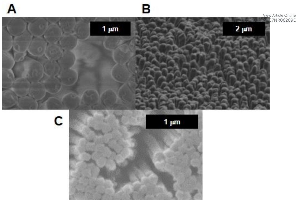
Figure 2. SEM images of Fe 3 O 4 -PNIPAm nanopillars (A) top view, (B) side view; (C) non-magnetic PNIPAm nanopillars top view.
