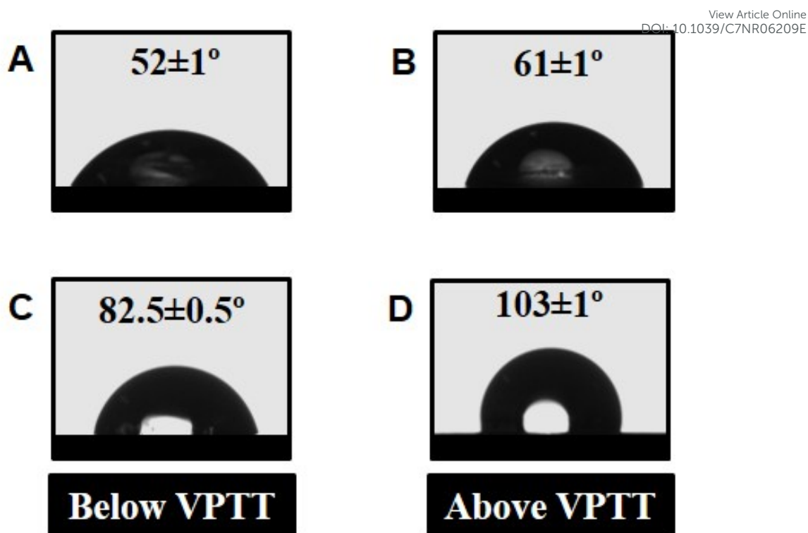
Figure 6. Contact angle of PNIPAm (A and B, 25 and 35°C, respectively) and Fe 3 O 4 -PNIPAm nanopillars (C and D, 25 and 35°C, respectively), nanopillars below and above VPTT. The nanopillars were supported on glass.
