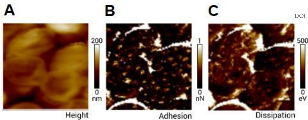
Figure 5. In-situ AFM three-dimensional (A) topographic images, (B) adhesion force and (C) dissipation at 35°C of Fe 3 O 4 -PNIPAm nanopillars surfaces. Scan size: 1 μm × 1 μm
