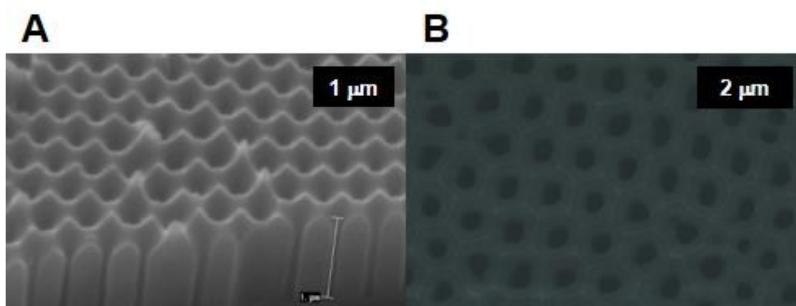
Figure 1. Morphological characterization of AAO nanoreactor by SEM. SEM allows to determine AAO template diameter and length. The dimensions of the nanoreactor were: \sim 1 \mu\text{m} (A) of pore length and 200 nm (B) of pore diameter.
