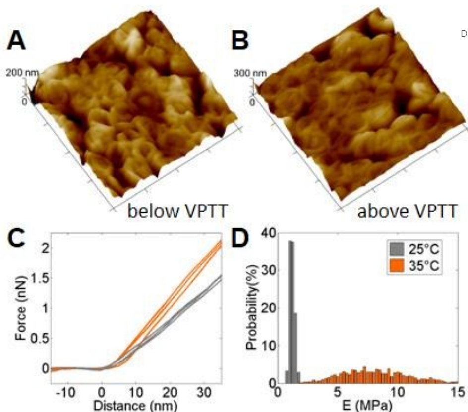
Figure 4. In-situ AFM three-dimensional topographic images of \text{Fe}_3\text{O}_4 -PNIPAm nanopillars surfaces (A) below and (B) above VPTT, (C) representative force-distance curves and (D) frequency histograms of the Young Modulus at 25°C (gray, Mean stiffness = 1.20 MPa, Std = 0.21 MPa, N = 714 force curves from 8 nanopillars) and 35°C (orange, Mean stiffness = 8.6 MPa, Std = 4.3 MPa, N = 1424 force curves from 8 nanopillars). All images were acquired in solution on PF-QNM mode; scan size: 2\ \mu\text{m} \times 2\ \mu\text{m} , z-scale indicated on each image.
