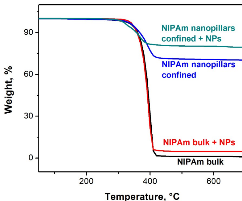
Figure 3. TGA profile for bulk and nanostructured (in confinement) \text{Fe}_3\text{O}_4 -PNIPAm; and bulk and nanostructured (in confinement) PNIPAm.
