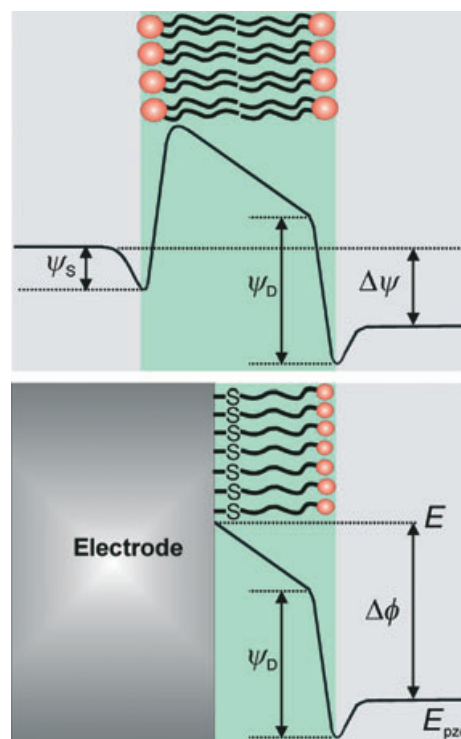
Fig. 1. Schematic presentation of the potential distribution at the membrane–solution interface (top) and at the electrode–SAM interface (bottom). \psi_s , \psi_D and \Delta\psi denote the surface potential, dipole potential and transmembrane potential, respectively; \Delta\phi is the difference between electrode potential ( E ) and the potential of zero charge ( E_{pzc} ).
