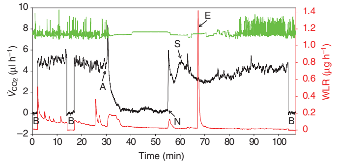
Fig. 3. Typical traces of a 25 min anoxia exposure at 25°C (single male fly, mass 0.793 mg). Black trace: rate of CO 2 emission (V CO 2 ); red trace: rate of water loss (WLR); green trace: activity (arbitrary units). A, initiation of anoxia; B, baseline (respirometer chamber switched out of circuit under program control); E, excretion event (which demonstrates the rapid response time for the water vapor signal); N, re-initiation of normoxia; S, secondary peak of CO 2 output.
