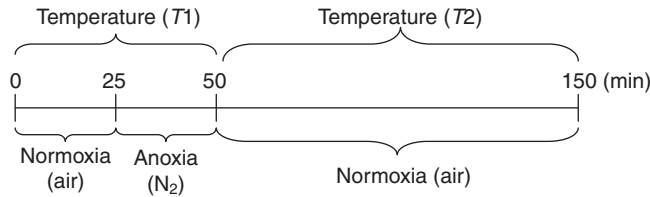
Fig. 2. Schema showing the protocol used in the second series of experiments. Time is in minutes. Temperature in the first 50 min (T1) was fixed at 20 or 30°C. For the first 25 min, flies were exposed to normoxic conditions. For the next 25 min flies were exposed to an anoxic atmosphere (pure nitrogen). Temperature in the last 100 min (T2) was also fixed at 20 or 30°C. T2 was the period allowed for recovery in normoxic conditions. Treatments were performed at 20/20; 20/30 and 30/20°C (T1/T2, respectively).
