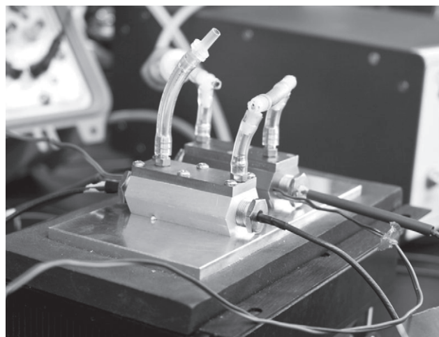
Fig. 1. Metal respirometry chambers (volume <1 ml) with sapphire windows at each end to allow photoelectric detection of activity used in all experiments. The chamber was in tight thermal contact with a temperature-controlled plate. Air entering the chamber was equilibrated to the chamber's temperature by traveling through a serpentine path milled into the upper metal surface of the metal block.
