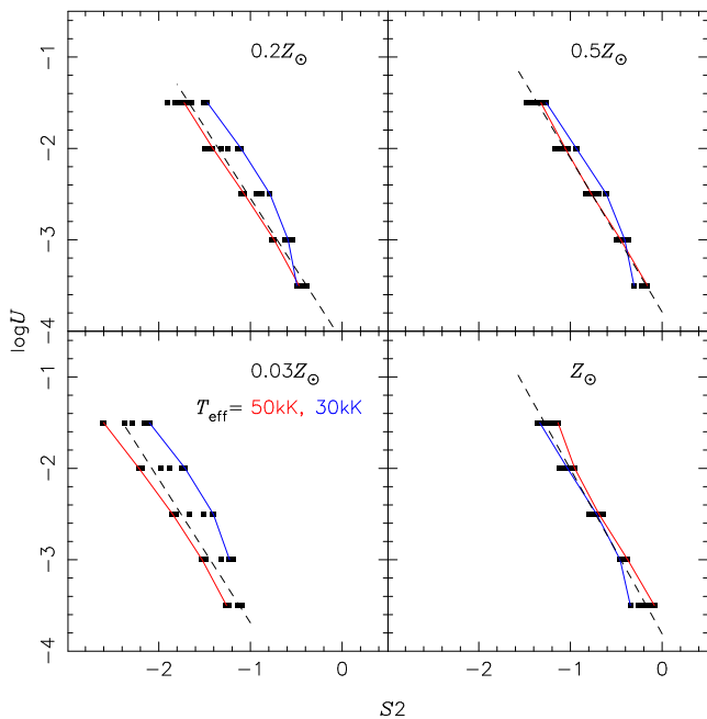
Figure 3. Logarithm of the ionization parameter ( \log U ) versus the line ratio S2 = \log[\text{S II}](\lambda\lambda 6717 + 31)/\text{H}\alpha for different values of metallicity ( Z/Z_{\odot} ) and different T_{\text{eff}} values, as indicated. Points, linked by solid lines, represent the results of our photoionization models (see Sect. 2) for T_{\text{eff}} values of 30 kK and 50 kK, as indicated. Dashed lines represent linear regression on the average of S2 values for each \log U , whose the coefficients are listed in Table 3.
