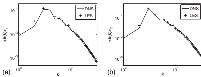
FIG. 4. Time averaged energy spectra for runs IIId (DNS: 256^3 , solid line) and IIII (LES: 64^3 , ++ ) at Ro=0.17 (top) and runs IIIId (DNS: 256^3 ) and IIIIL (LES: 64^3 ) at Ro=0.35 (bottom). Time averaging is performed from t=25 to t=45 for both simulations. Note the good agreement except possibly near k=2 corresponding to the forcing scale, indicative of a lack of adjustment of the LES at that scale, in particular for the perpendicular spectra (see Fig. 5).
