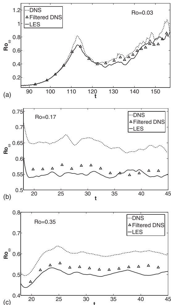
FIG. 6. Temporal evolution of the micro-Rossby-number Ro_\omega in flows with Ro=0.03 (top), Ro=0.17 (middle), and Ro=0.35 (bottom) for DNS on 256^3 grid points (dashed line), filtered data of the DNS to a 64^3 grid (triangles), and LES (solid line) on a 64^3 grid. Note again the different scale on the axes, in particular for the lowest Rossby number in which case Ro_\omega approaches unity as the inverse cascade develops and energy and turbulence intensity grow.
