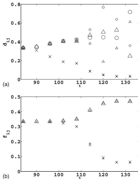
FIG. 9. Measuring anisotropy through the diagonal components of the tensors of dimensionality (top) and circicity (bottom) [see Eq. (15)], with directions 1-1, 2-2, and 3-3 given respectively with triangles, circles, and crosses. Small symbols correspond to the DNS Ir and large symbols are for the LES II at Ro=0.03 . Note that the latter is much less scattered than the former for the components in the horizontal plane, and that it remains close to its isotropic value of 1/3 for a longer time till the onset of the inverse cascade of energy, time after which anisotropy develops for both coefficients.
