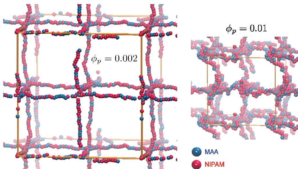
Figure 6. The scheme represents the molecular model of polymer network used in our theoretical calculations. Random NIPAM- co -MAA copolymer chains are crosslinked at nodal units. Each crosslink joins six 25 segment-long chains; the polymer segment length is 0.5 nm. The two panels correspond to different volume fractions of polymer inside a single microgel, \phi_p . These volume fractions represent the relatively compact ( \phi_p=0.01 ) and swollen ( \phi_p=0.002 ) microgels observed in Fig. 2 for 5 mM salt solutions and at temperatures lower than the VPTT. Orange tubes enclose the calculation box; full-3D periodic boundary conditions are applied in the calculations.
