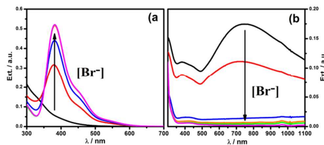
Figure 1. Extinction spectra of 0.1 mM \text{HAuCl}_4 reactive solutions with increasing bromide ion concentration: (black) 0.01 mM, (red) 0.05 mM, (blue) 1 mM, (orange) 5 mM, (green) 7.5 mM, (pink) 50 mM; (a) before and (b) 15 min after \text{H}_2\text{Q} addition ( [\text{H}_2\text{Q}]_{\text{final}}=0.15 mM, \text{pH}=6.5 ).
