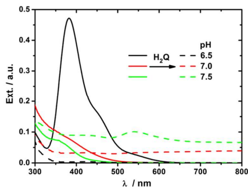
Figure 3. Extinction profiles for 0.1 mM \text{HAuCl}_4 , 50 mM KBr solutions at different pH values: (black) 6.5, (red) 7, and (green) 7.5, before (solid lines) and 15 min after (dashed lines) \text{H}_2\text{Q} addition. Final \text{H}_2\text{Q} concentration: 0.15 mM.
