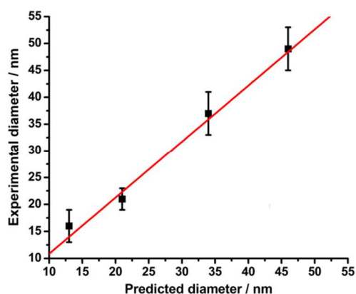
Figure 8. Experimental AuNPs diameter determined by TEM with its corresponding dispersion bars vs. calculated diameter by using as inputs the seed size and the [Au(I)]/[seeds] ratio.
