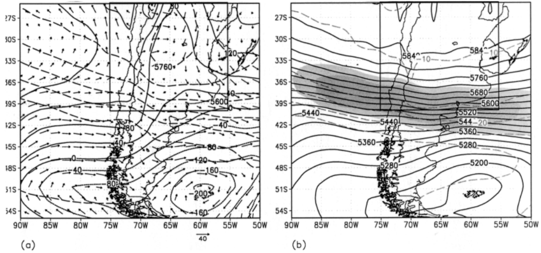
FIG. 8. Same as in Fig. 2 except for 1200 UTC 10 Aug 1999.
