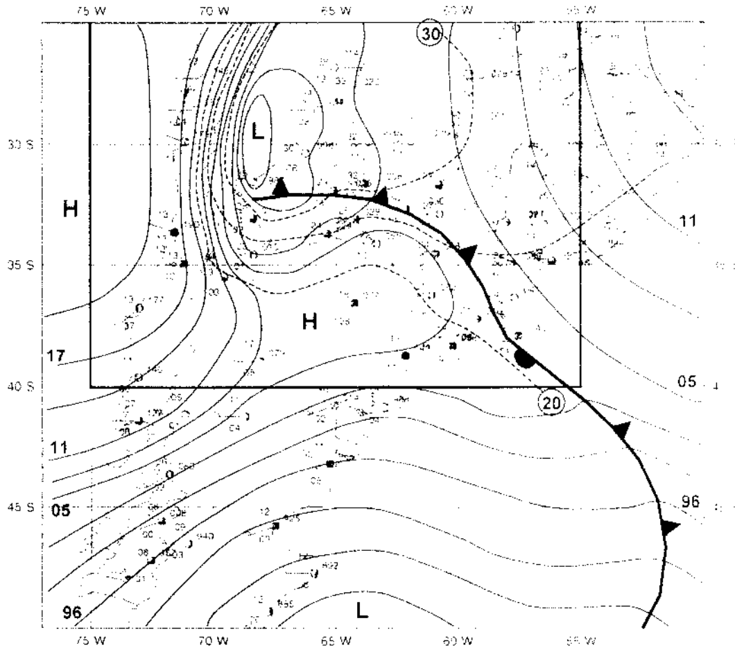
FIG. 4. Hand-drawn analysis corresponding to 1800 UTC 5 Aug 1999. Isobars (solid lines) at 3-hPa intervals and isotherms (dashed lines) at 5°C intervals. Symbols used have their usual meaning. Wind barbs are in kt. Solid rectangle corresponds to the region shown in Fig. 1.
