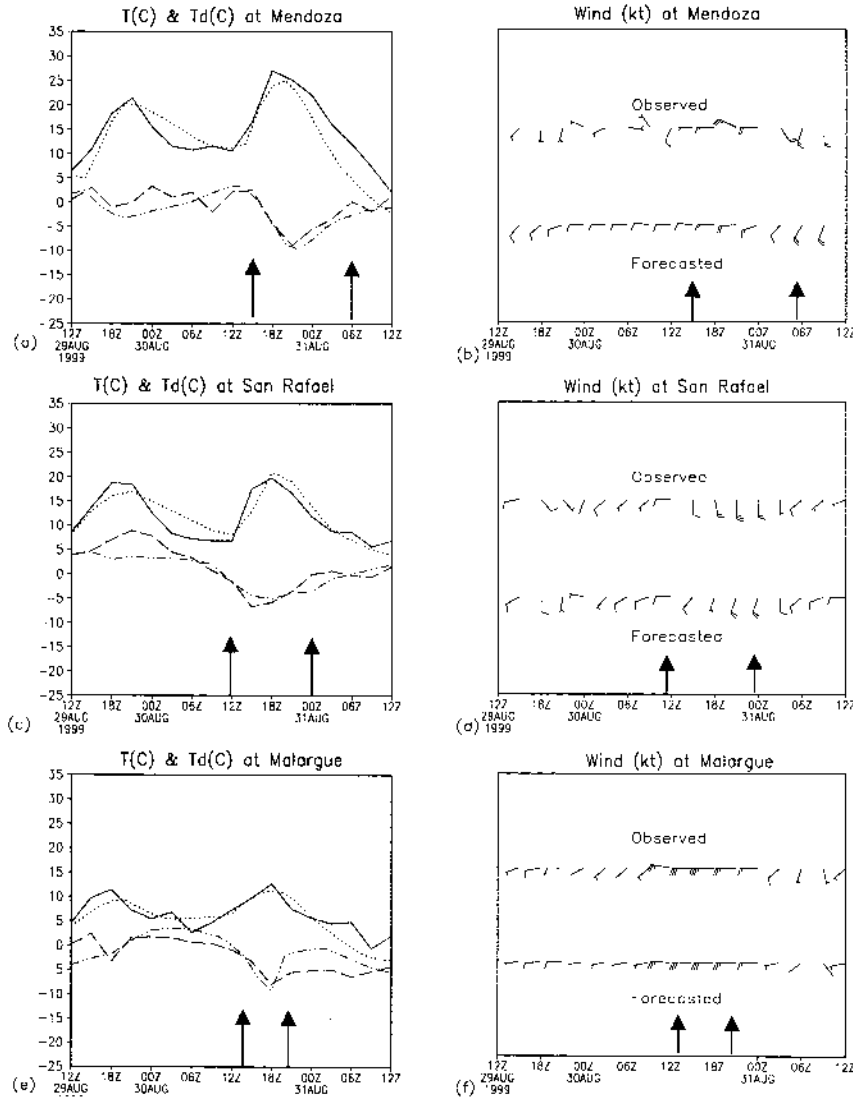
FIG. 13. As in Fig. 5 except for 30 Aug 1999.
