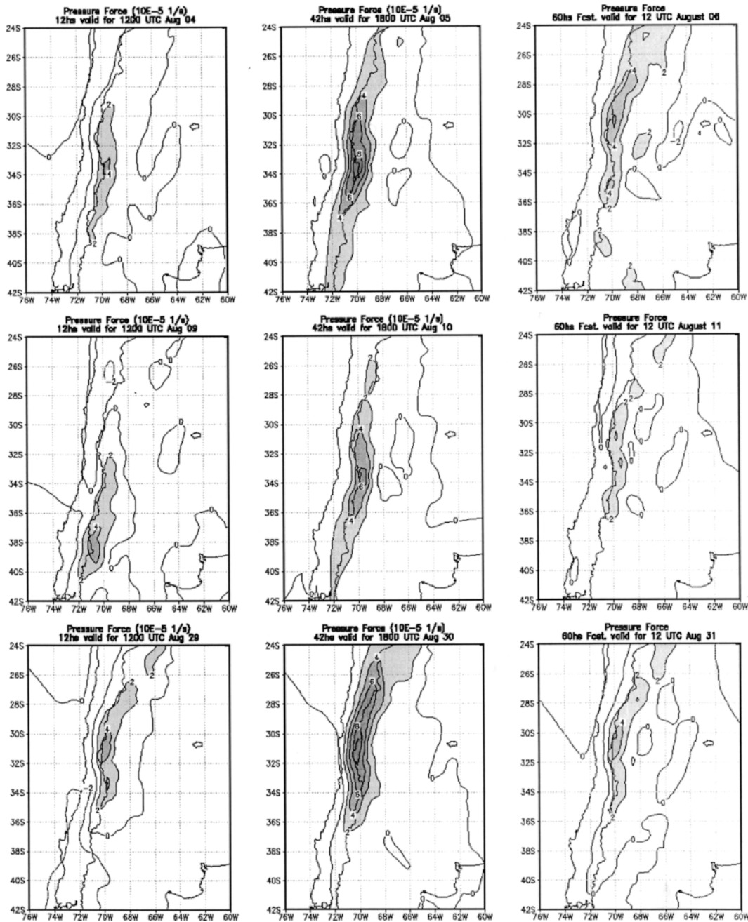
FIG. 22. Magnitude of the pressure gradient force ( 10^{-5} \text{ m s}^{-2} ) at the lowest model level obtained from the model simulations for the indicated days and hours. Values higher than 2 \cdot 10^{-5} \text{ m s}^{-2} are shaded.
