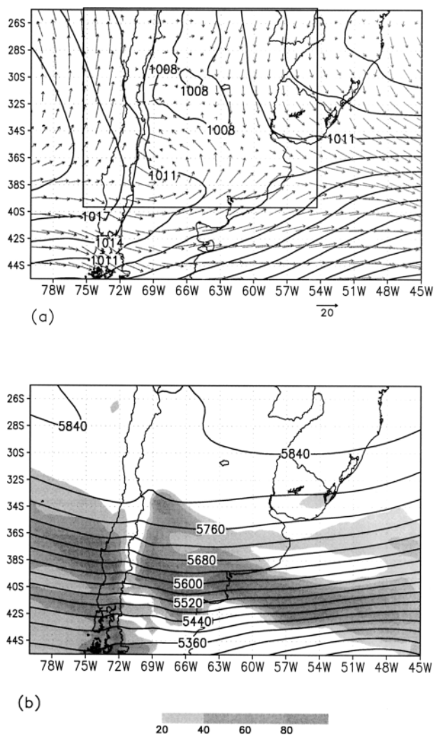
FIG. 15. Same as in Figs. 14a and 14b except for 1800 UTC 10 Aug 1999.
