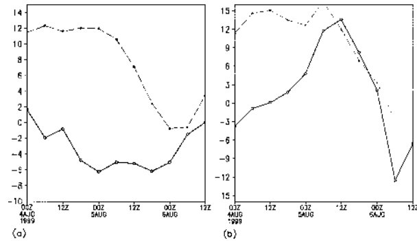
FIG. 20. Difference of the equivalent potential temperature (K) between the 500- and 1000-hPa levels (dashed lines) and magnitude of the vertical velocity ( \text{hPa s}^{-1} ) at (a) 34^{\circ}\text{S} , 75^{\circ}\text{W} and (b) 34^{\circ}\text{S} , 68^{\circ}\text{W} simulated by the Eta–CPTEC model.
