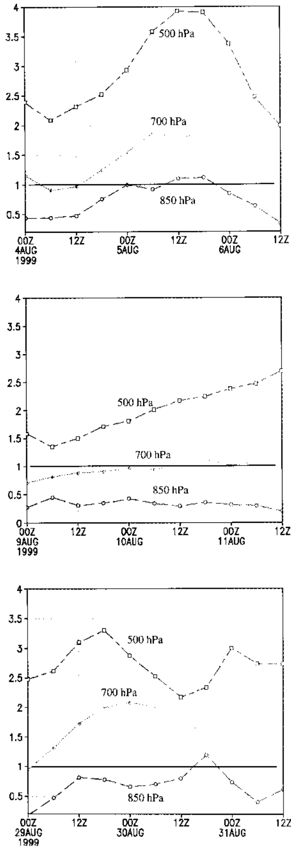
FIG. 21. Temporal evolution of Fr, obtained from the diagnostics of the Eta-CPTec model at 34°S, 75°W at 850, 700, and 500 hPa for the situations of (a) 5, (b) 10, and (c) 30 Aug 1999.
