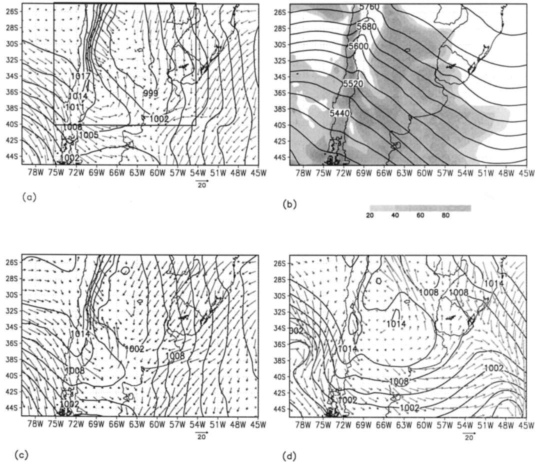
FIG. 16. Same as in Fig. 14 except for 30 Aug 1999.
