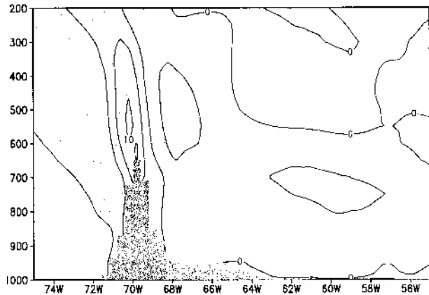
FIG. 19. Same as in Fig. 18 except for 1200 UTC 10 Aug (36-h integration).
