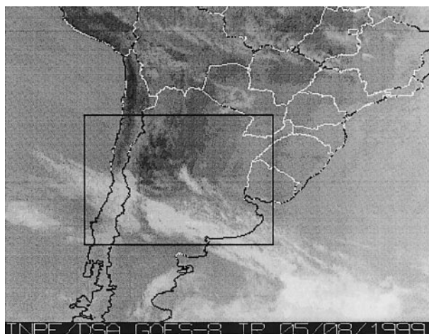
FIG. 7. GOES infrared satellite image corresponding to 1800 UTC 5 Aug 1999. Dark rectangle corresponds to the region shown in Fig. 1.
