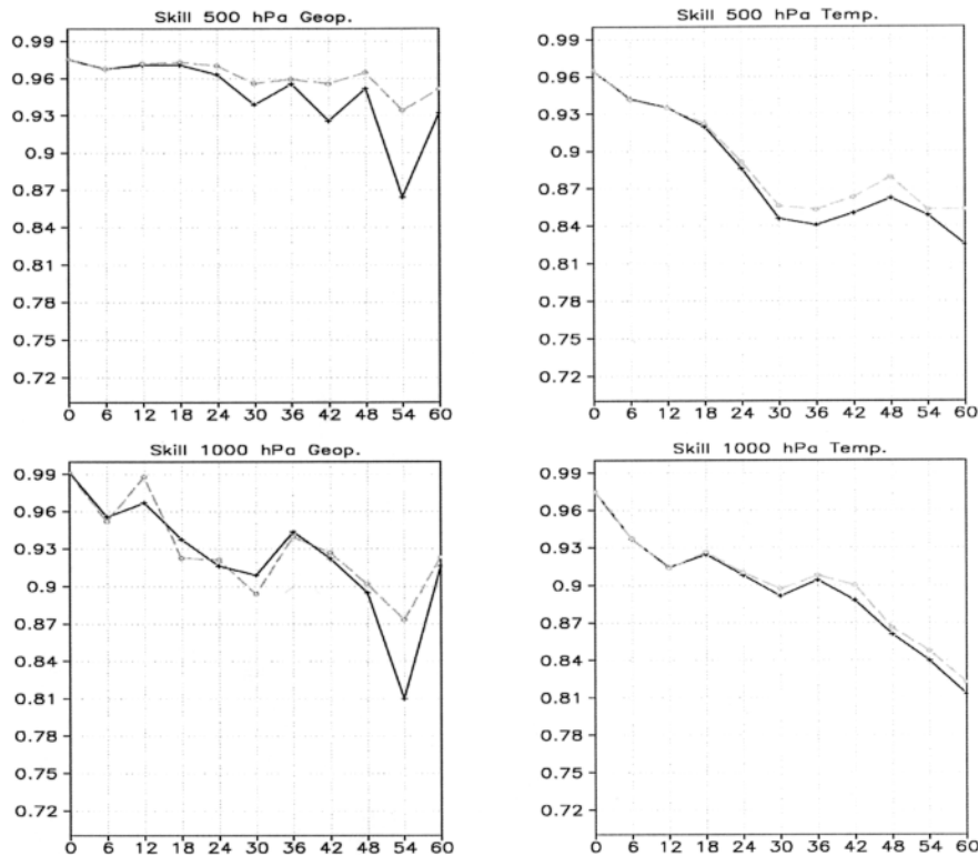
FIG. 17. Mean anomaly correlation between model outputs, forecasts, and simulations, obtained by the Eta-CPTEC model and NCEP analysis for (left) geopotential height and (right) temperature at the (above) 500- and (below) 1000-hPa levels. The solid lines correspond to the score averaged over the three situations for 42-h forecasts (i.e., initiated 42 h before the appearance of the zonda wind). The dashed lines correspond to the simulations (analyzed boundary conditions) obtained for the same period. Time on the x axis represents hours of integration.
