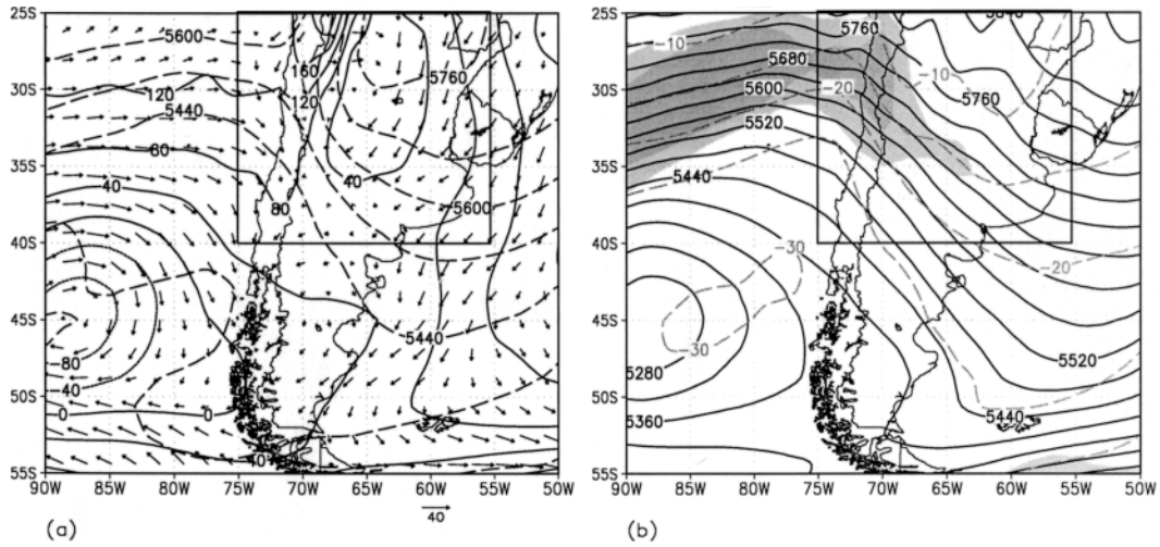
FIG. 11. Same as in Fig. 2 except for 1200 UTC 30 Aug 1999.
