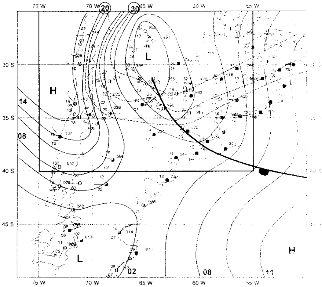
FIG. 12. Same as in Fig. 4 except for 1800 UTC 30 Aug 1999.
