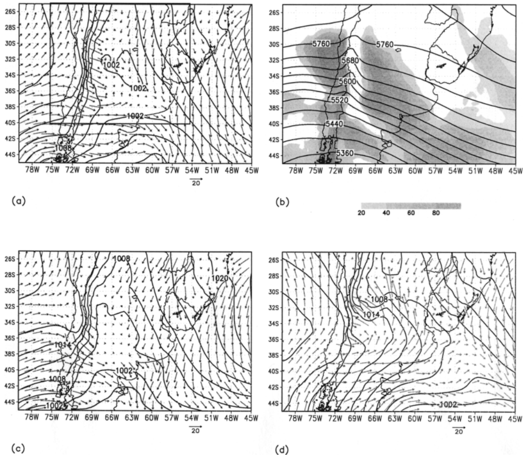
FIG. 14. The 42-h forecast valid for 1800 UTC 5 Aug 1999: (a) sea level pressure (solid lines, every 3 hPa) and wind at anemometer level (vectors, kt), (b) geopotential height at 500-hPa level (solid line, every 40 gpm) and cloudiness (% , shaded according to grayscale shown), (c) same as in (a) except for 36-h forecast valid for 1200 UTC 5 Aug 1999, and (d) same as in (a) except for 60-h forecast valid for 1200 UTC 6 Aug 1999.
