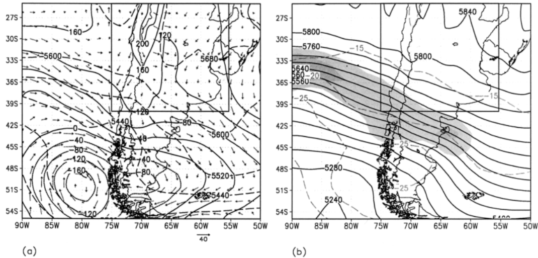
FIG. 2. Meteorological situation corresponding to 1200 UTC 4 Aug 1999 (NCEP analysis). (a) geopotential height of the 1000-hPa level (solid line, gpm), 500–1000-hPa thickness (dashed line, gpm), and winds at anemometer level (vectors; in kt). (b) The 500-hPa geopotential height (solid line, gpm), temperature (dashed line, °C), and winds (light shading 80–120-kt interval, darker shading >120 kt). Solid rectangle corresponds to the region shown in Fig. 1.
