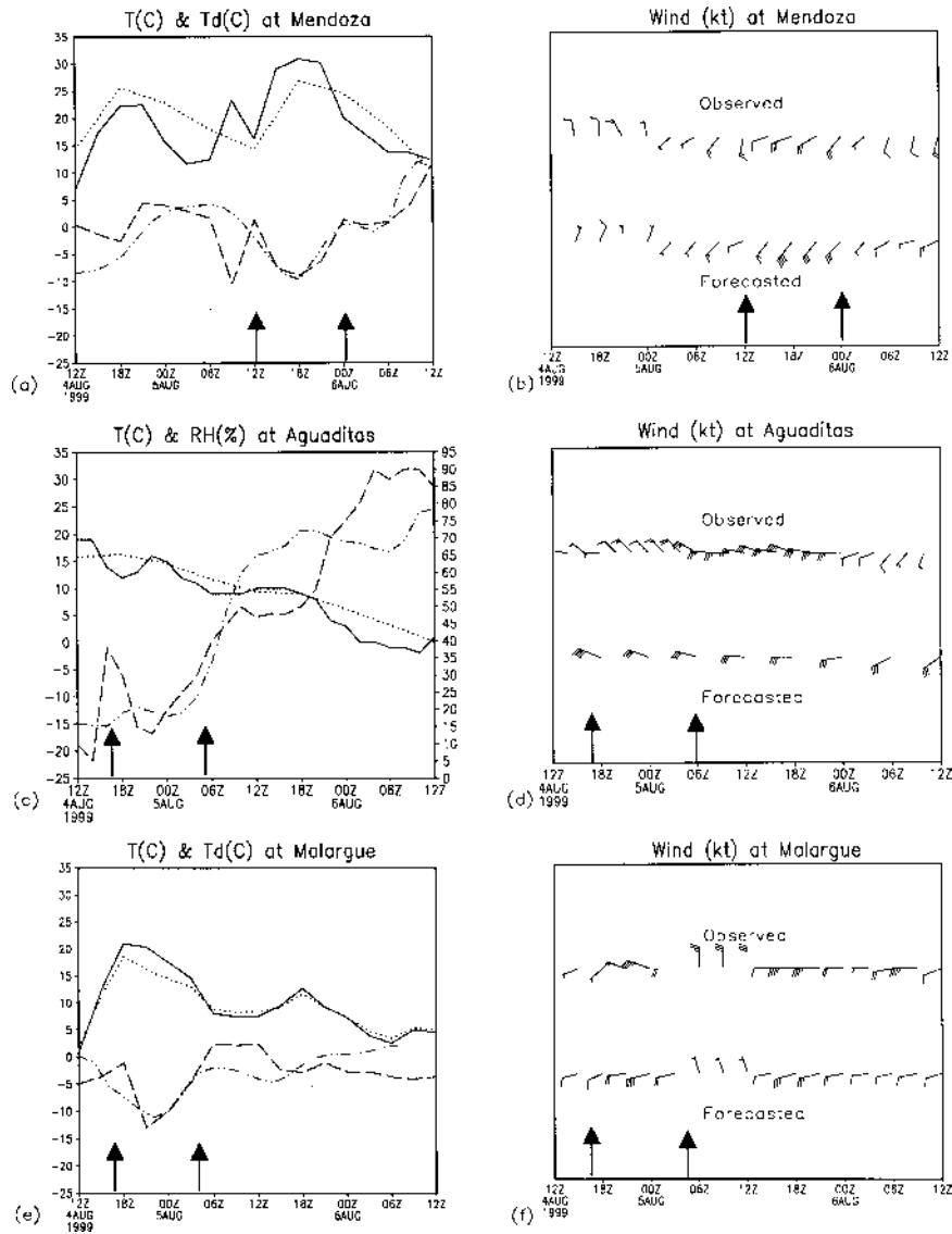
FIG. 5. Temporal evolution of observed and forecast (Eta-CPTEC model) meteorological variables at the indicated stations (see geographic location in Fig. 1). (a), (e) Observed temperature ( ^{\circ}\text{C} , solid lines), observed dewpoint temperature ( ^{\circ}\text{C} , dashed lines), forecast temperature ( ^{\circ}\text{C} , dotted lines), and forecasted dew point temperature ( ^{\circ}\text{C} , dot-dot-dash lines). (c) Observed temperature ( ^{\circ}\text{C} , solid lines), observed relative humidity (% , dashed lines), forecast temperature ( ^{\circ}\text{C} , dotted lines), and forecasted relative humidity (% , dot-dot-dash lines). (b), (d), (f) Observed winds (kt) and forecasted winds (kt). Arrows in (a)–(c) indicate zonda starting and terminating times, respectively.
