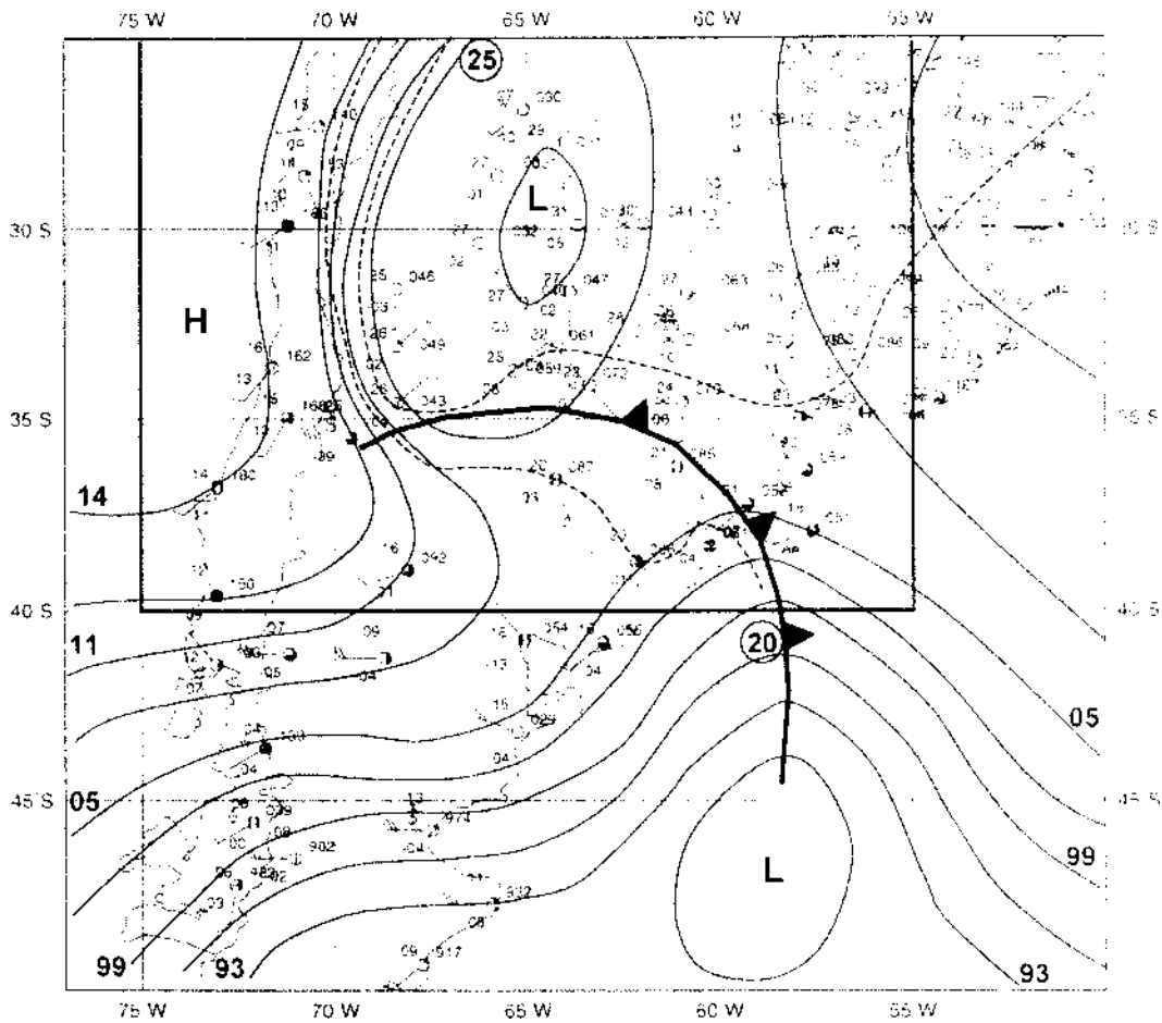
FIG. 9. Same as in Fig. 4 except for 1800 UTC 10 Aug 1999.
