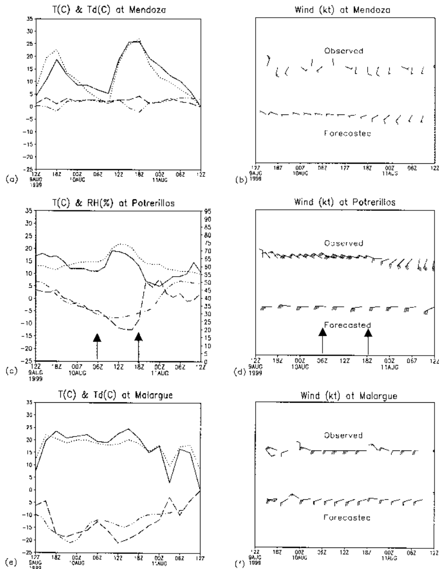
FIG. 10. Same as in Fig. 5 except for 10 Aug 1999.
