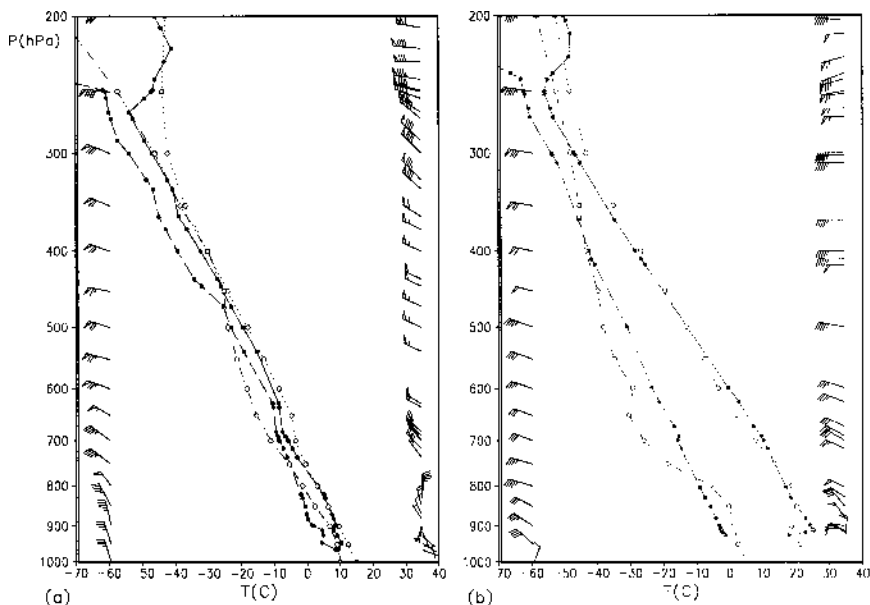
FIG. 6. Aerological soundings at 1200 UTC on 5 Aug 1999 at (a) Quintero and (b) Mendoza stations. The profiles correspond to the observed temperature ( ^{\circ}\text{C} , solid line) and dewpoint temperature ( ^{\circ}\text{C} , dashed line), and those forecast by the Eta-CPTEC model at the nearest grid point (temperature in dotted lines and dewpoint temperature in dot-dot-dash lines). Observed (forecast) wind profile is shown on the right (left) side. Winds are in kt.
