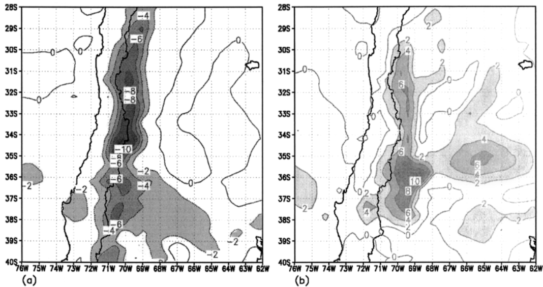
FIG. 23. Difference in the 925-hPa wind magnitude between the control experiment and the one in which the Andes height was multiplied by a factor of 0.75. (a) After 42 h of integration, valid for 1800 UTC 5 Aug (values lower than -2 \text{ m s}^{-1} are shaded). (b) After 42 h of integration, valid for 1800 UTC of 10 Aug. Values higher than 1 \text{ m s}^{-1} are shaded.
