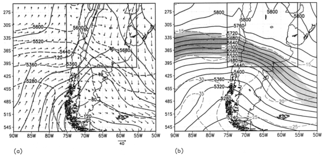
FIG. 3. Same as in Fig. 2 except at 1200 UTC 5 Aug 1999.
