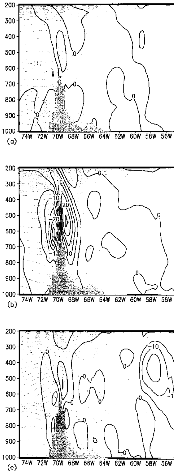
FIG. 18. Vertical cross sections of the equivalent potential temperature (K, dashed lines), vertical velocity ( \text{hPa s}^{-1} , solid lines) at
