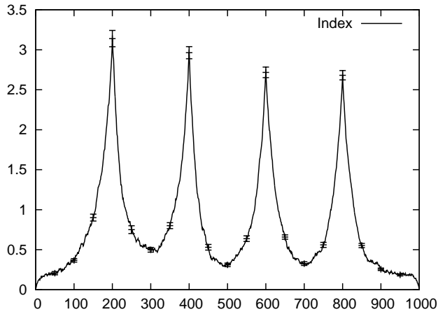
Figure 3: Distance between adjacent hyperplanes. The line shows the average value over 30 trials while the bars show their standard error.
