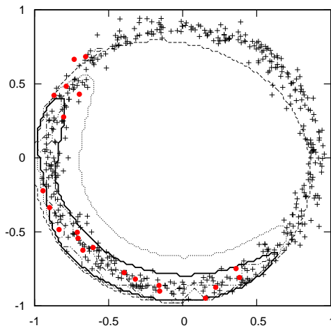
Figure 2: Selected area by OC-TA-SVM for time t = 200 for various values of \sigma . Big values of \sigma are shown with dotted and dashed lines. A low value is shown with a dashed and double point line, and an approximate optimal value with a thick line. The points from t = 190 to t = 210 are indicated in red.
