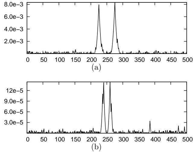
Figure 5: Index obtained with OC-TA-SVM for an example sequence with s = 25 (a) and another with s = 10 (b).
