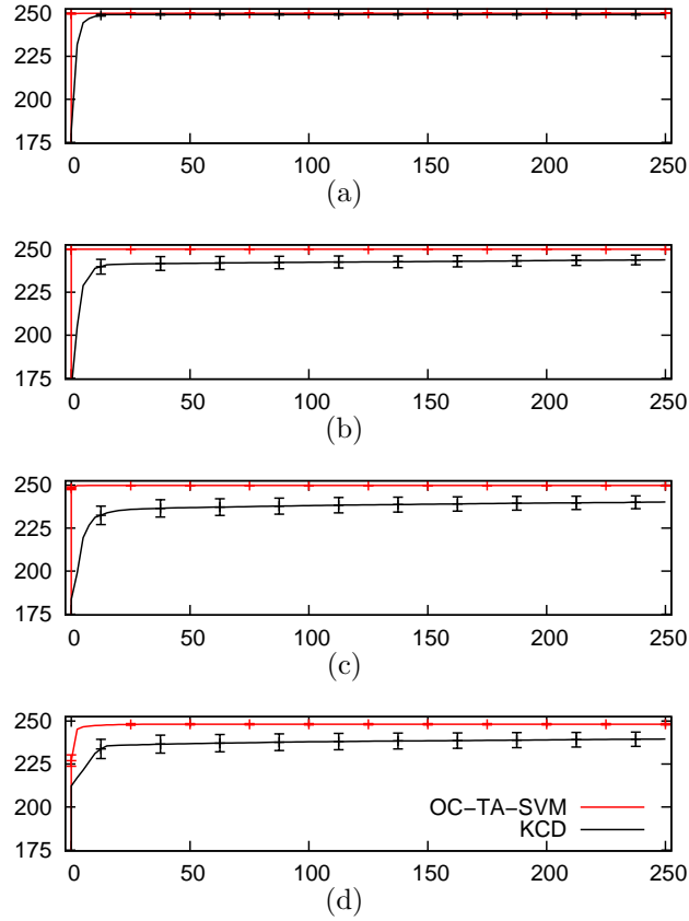
Figure 4: Number of correctly detected changes as a function of wrongly detected ones, for the no noise (a), 10% (b), 20% (c) and 30% noise cases (d). Bars indicate standard error.
