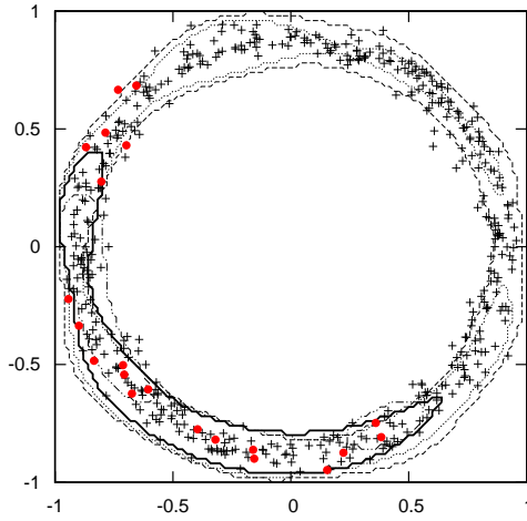
Figure 1: Selected area by OC-TA-SVM for time t = 200 for various values of \gamma . Big values of \gamma are shown with dotted and dashed lines. A low value is shown with a dashed and double point line, and an approximately optimal value with a thick line. The points from t = 190 to t = 210 are shown in red.
