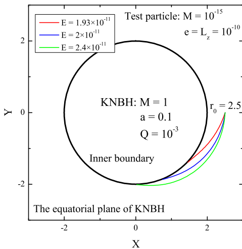
FIG. 3.— The trajectories of a test particle ( m = 10^{-15} , and e = L_z = 10^{-10} ) on the equatorial plane falling into a KNBH ( M = 1 , a = 0.1 , and Q = 10^{-3} ) from r_0 = 2.5 to the inner boundary ( r = r_g ) for E = 1.93 \times 10^{-11} , 2 \times 10^{-11} , and 2.4 \times 10^{-11} .
