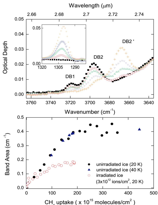
FIG. 6. (Color online) Top: Change in the dangling bonds upon adsorption of methane in unirradiated ice at 20 K. The inset shows the \sim 1300 \text{cm}^{-1} band during adsorption. The curves correspond to methane uptake of 0, 10.0, 53.6, 93.3, and 165.2 in ML units (1 ML = 10^{15} \text{CH}_4/\text{cm}^2 ). Bottom: Increase in the band area of the shifted dangling bond feature at 3669 \text{cm}^{-1} with increasing methane uptake. Gaussian fits were applied to deconvolute the features after subtraction of a curved continuum, as shown in Fig. 1.
