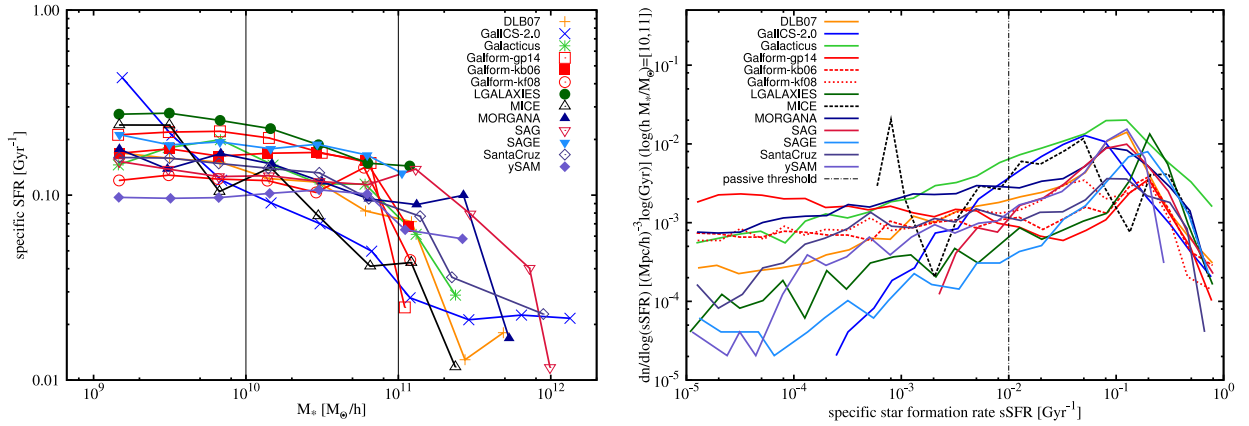
Figure 9. sSFR of star-forming galaxies at redshift z = 0 . The left-hand panel shows the SFR per stellar mass as a function of stellar mass M_* ; points represent mean values binned in both the y and x direction for the star-forming sequence of galaxies. The right-hand panel serves as a proxy for the (omitted) error bars: it shows the distribution of sSFR for galaxies in the mass range M_* \in [10^{10}, 10^{11}] h^{-1} M_\odot (indicated by the two vertical lines); the vertical dashed line indicates our choice for the passive galaxy fraction threshold.
